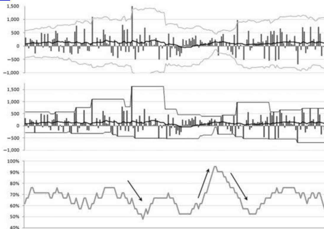
Figure 12.7 Three Control Charts
