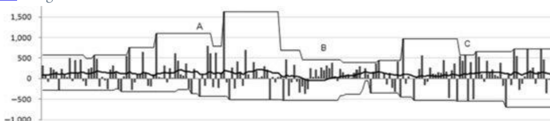
Figure 12.6 Range Control Chart
