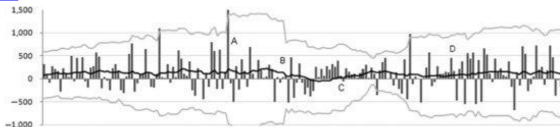
Figure 12.5 A Standard Deviation Control Chart
