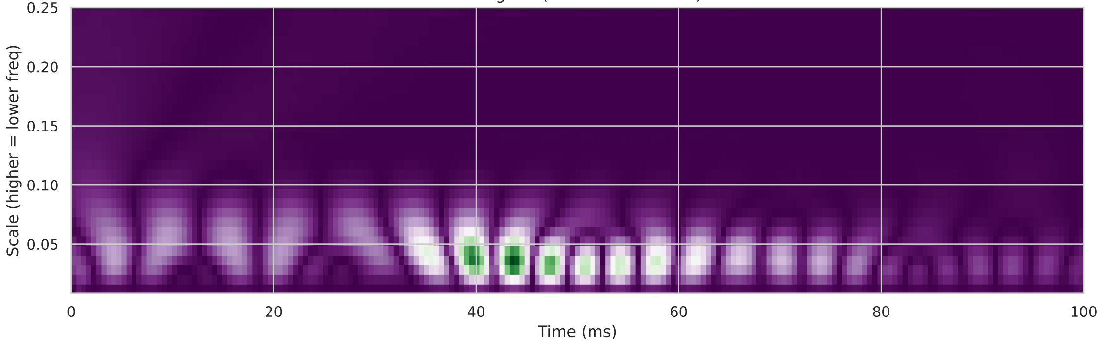
Scalogram (CWT - Mexican hat)
