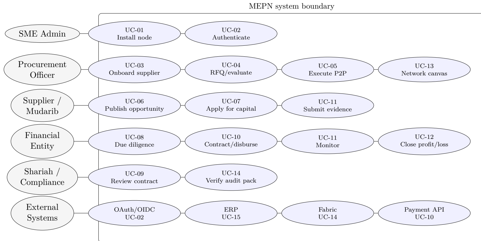
Figure 2: Use case diagram for MEPN showing actor-oriented use case groups
