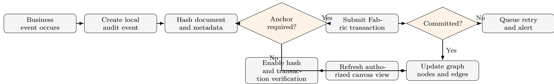
Figure 6: Activity diagram - network canvas and audit anchoring
