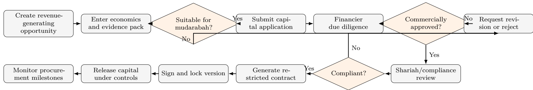
Figure 4: Activity diagram - mudarabah application and approval
