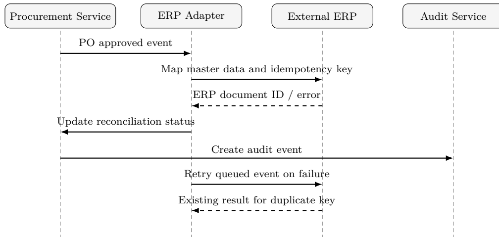
Figure 10: Sequence diagram - external ERP integration
