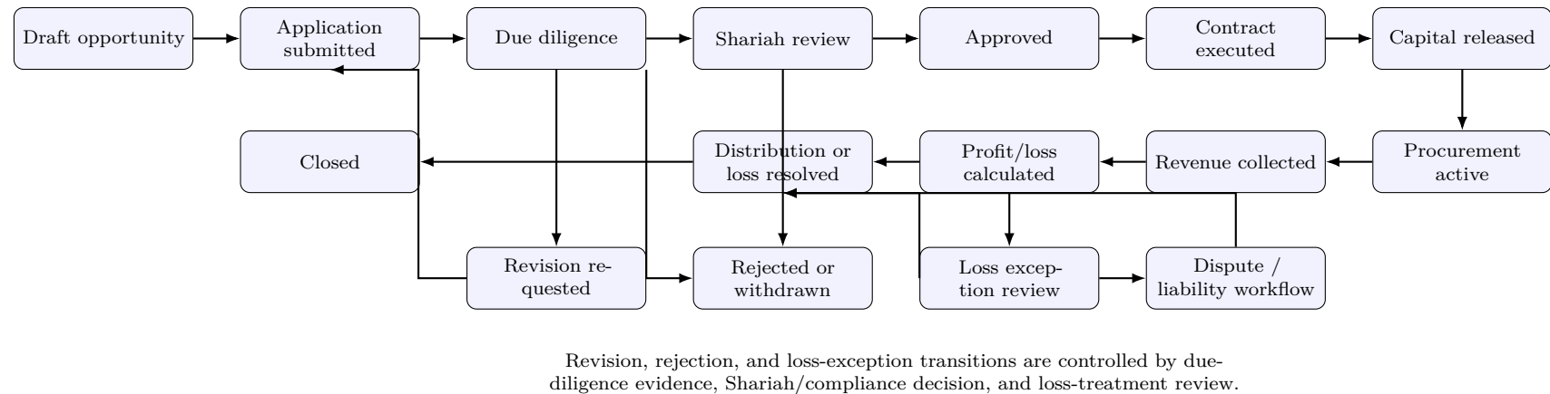
Figure 8: State machine - mudarabah application and contract lifecycle
