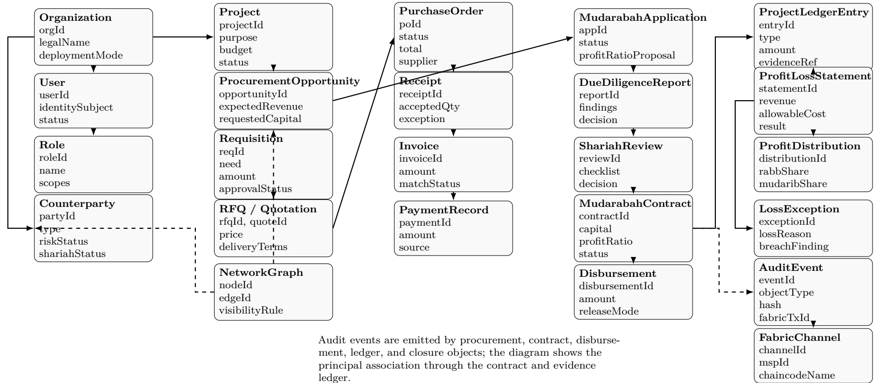
Figure 7: Domain class diagram showing principal classes and associations
