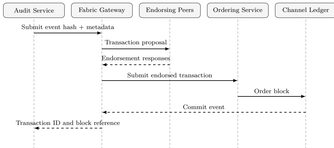
Figure 11: Sequence diagram - Fabric event anchoring
