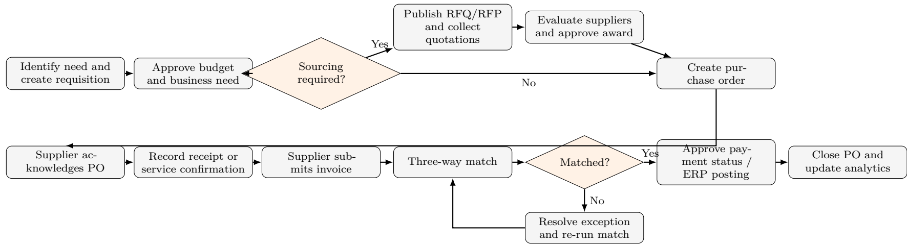
Figure 3: Activity diagram - procurement workflow
