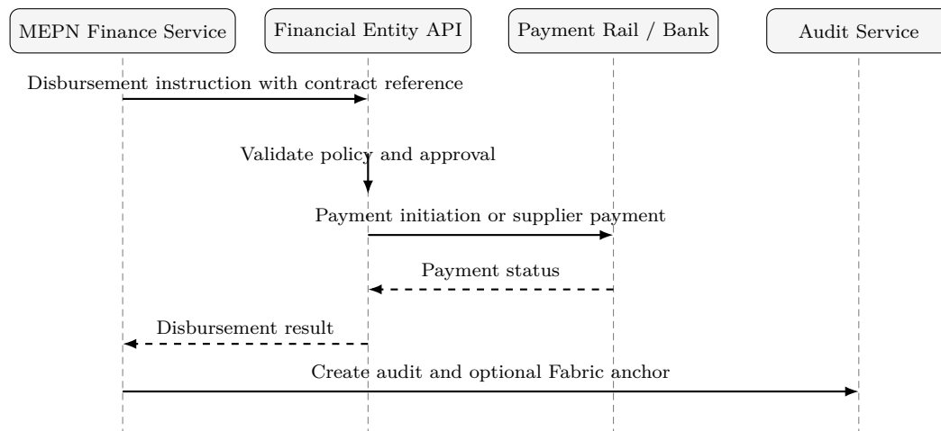
Figure 12: Sequence diagram - external financial entity disbursement API
