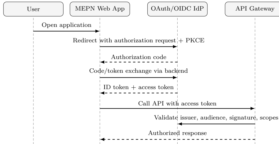
Figure 9: Sequence diagram - OAuth/OIDC login
