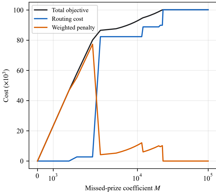
Cost decomposition with relaxed route budgets
