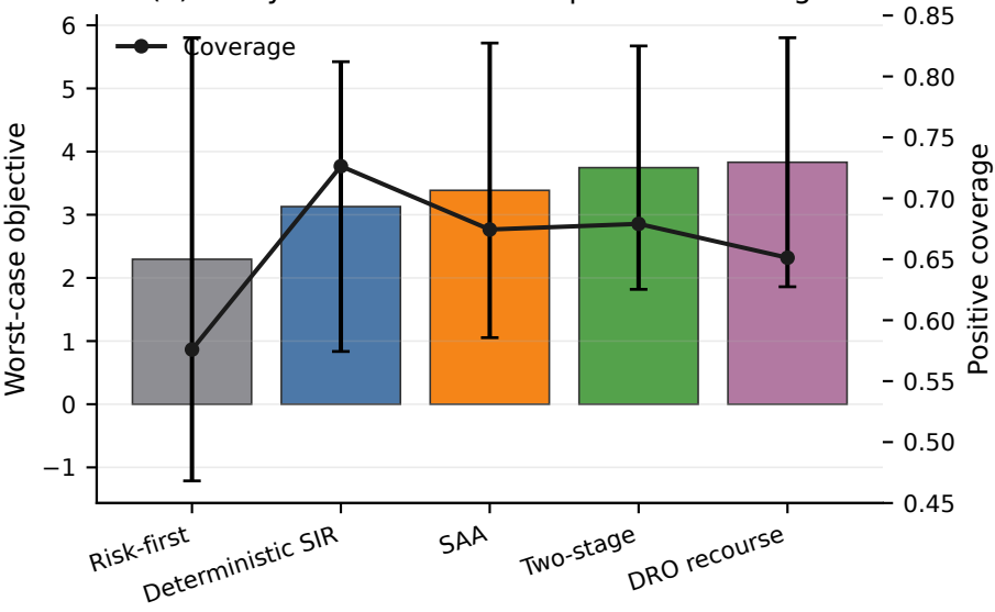
(a) Policy value and verified-positive coverage
