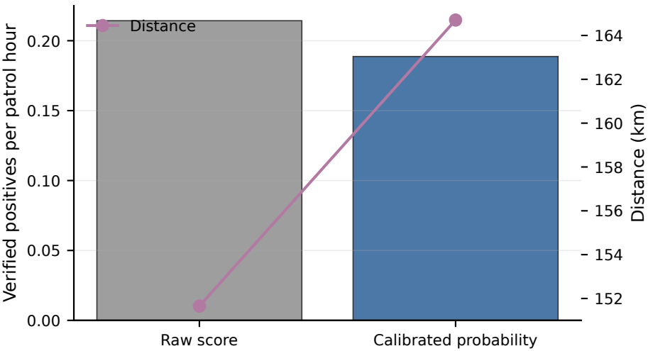
(c) Rank-preserving calibration and route outcomes
