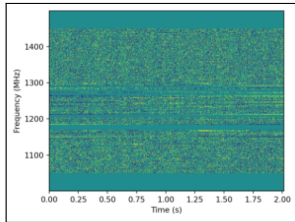
Negative (RFI/noise) peak = 2.8\sigma
