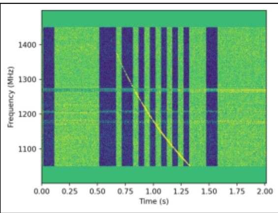
Real FRB, detectable peak = 26.5\sigma
