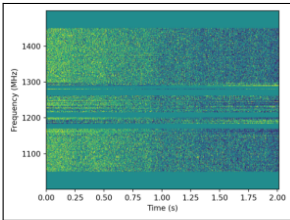
Real FRB, below noise floor peak = 1.9\sigma
