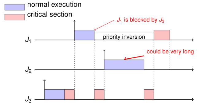
Fig. 3. Priority inversion and its effects [?]
