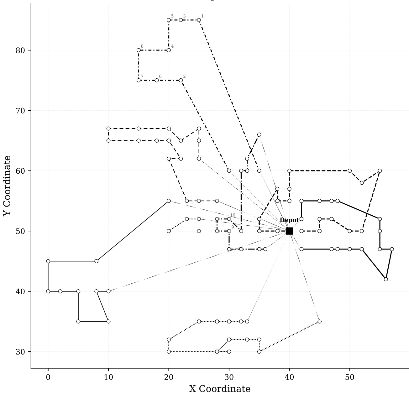
ACO Route Map (100 Customers)
