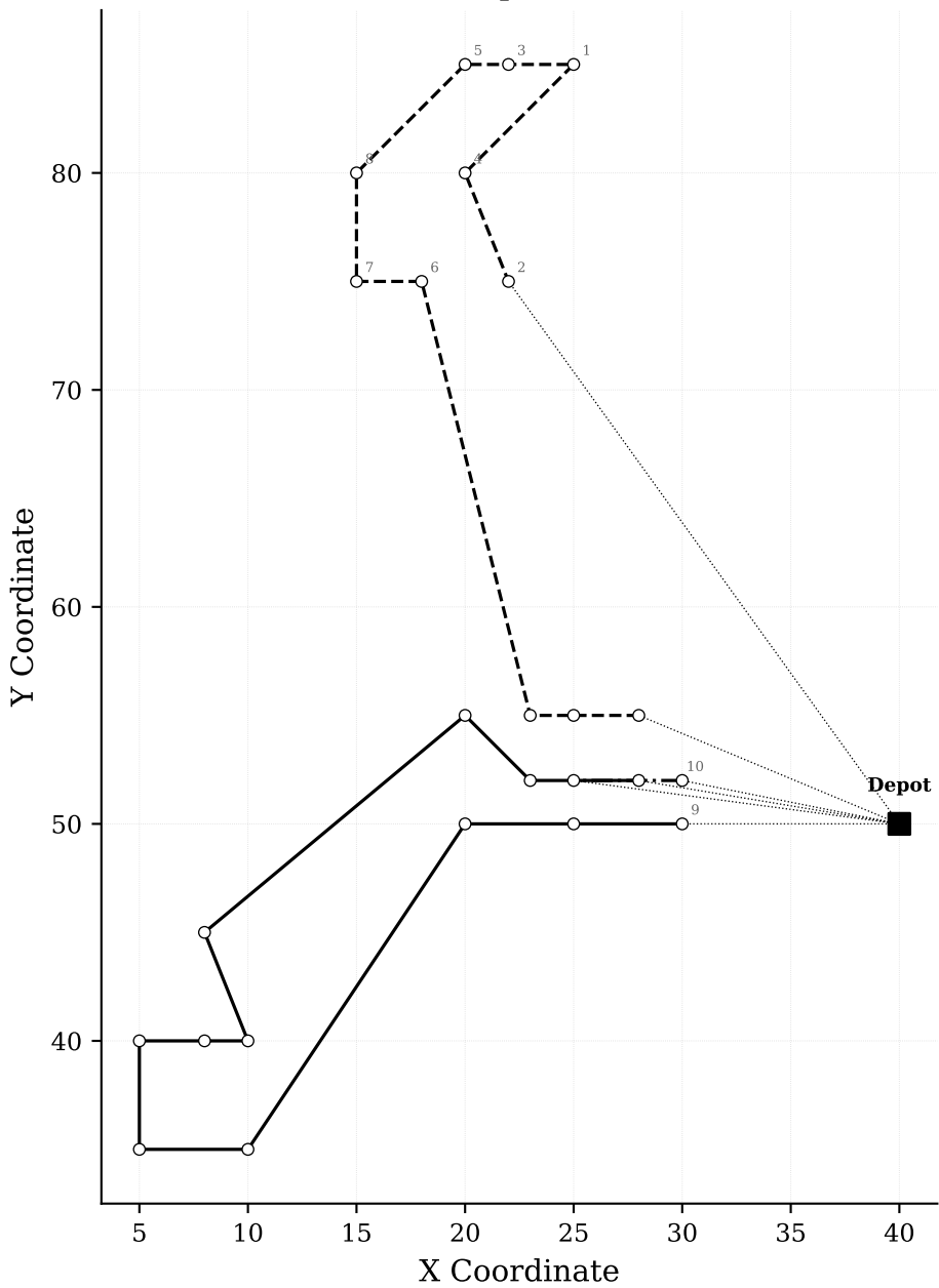
ACO Route Map (25 Customers)
