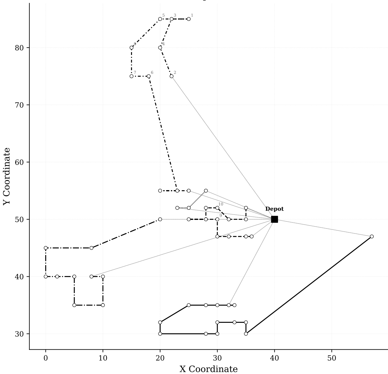
ACO Route Map (50 Customers)
