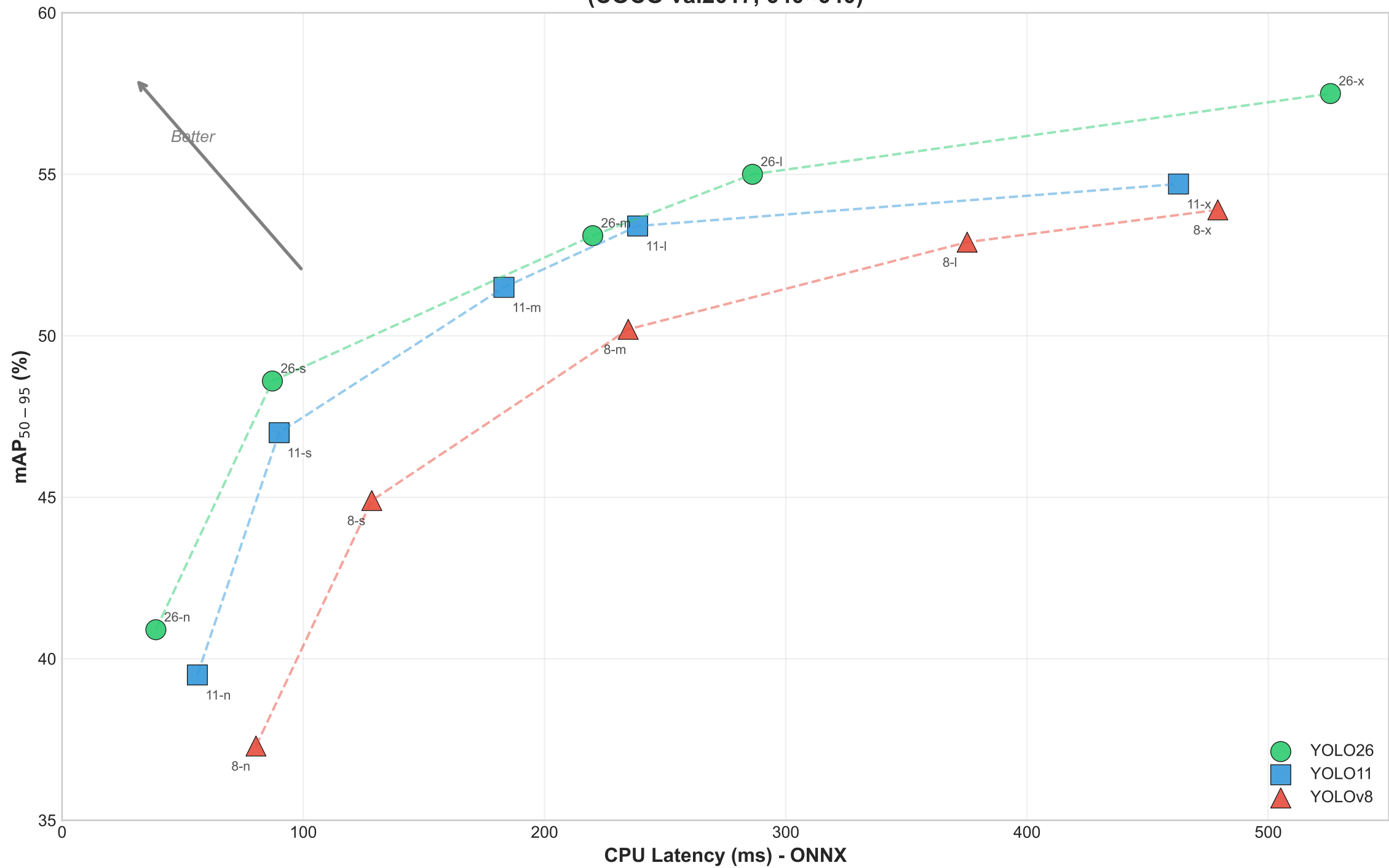
YOLO Models: Accuracy vs Speed Trade-off (COCO val2017, 640×640)
