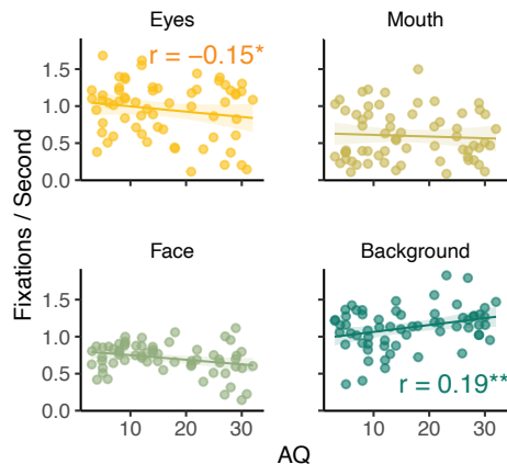
Autism Spectrum Quotient
