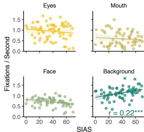
Social Interaction Anxiety
