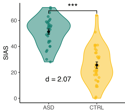
Social Anxiety by Group
