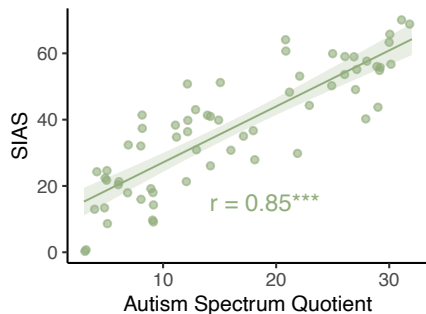
Social Anxiety and AQ
