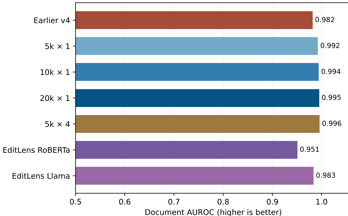
Ranking quality on the pure held-out set
