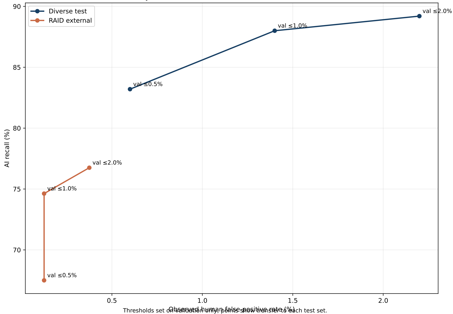
Qwen decision threshold trade-off
