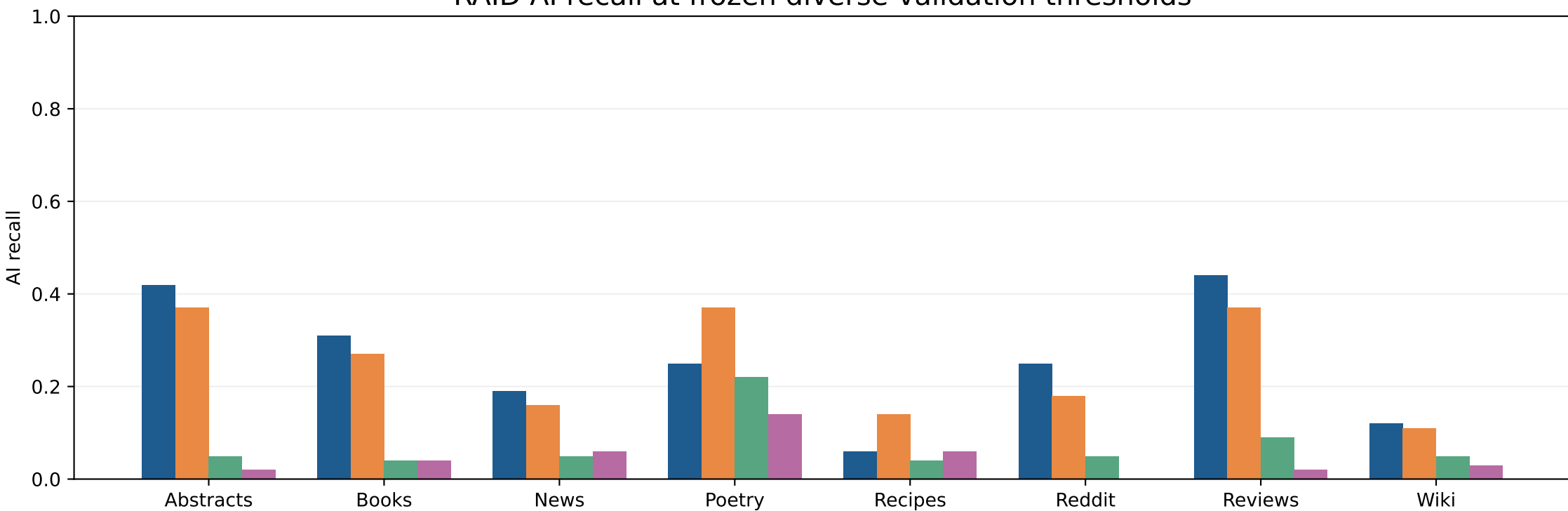
RAID AI recall at frozen diverse-validation thresholds
