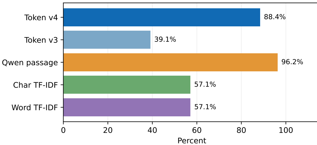
AITDNA mixed: AI token recall
