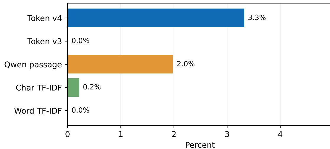
CoAuthor: AI token recall
