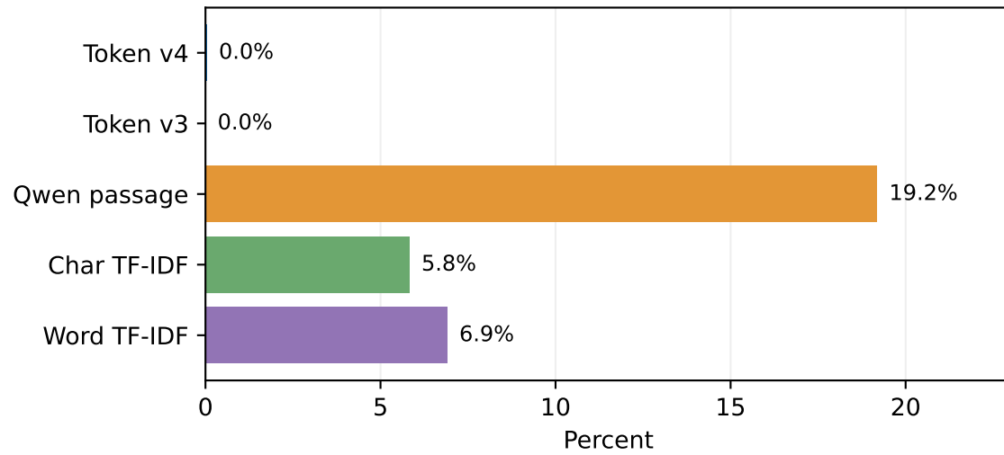
V4 synthetic: human token FPR
