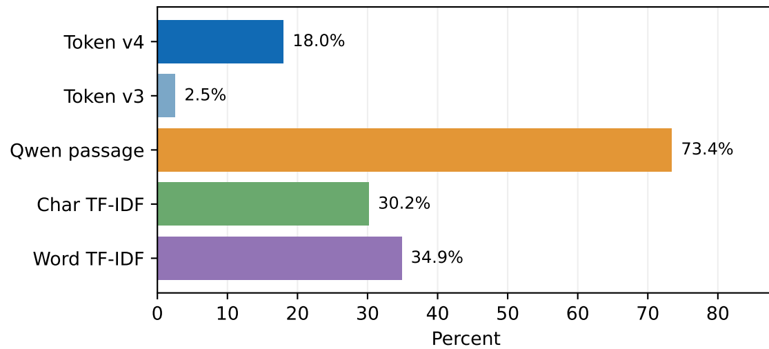
AITDNA mixed: human token FPR
