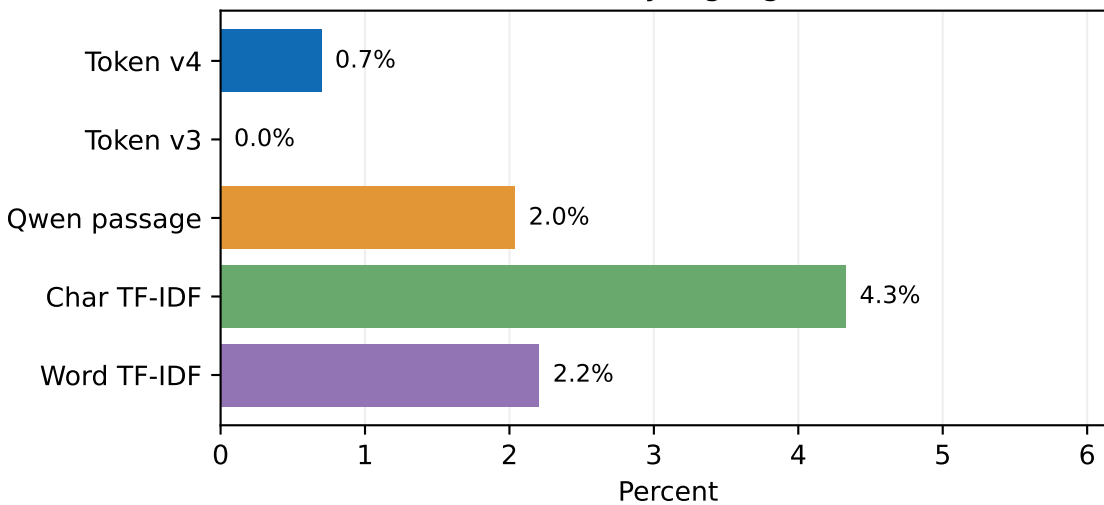
Locked human: docs falsely highlighted
