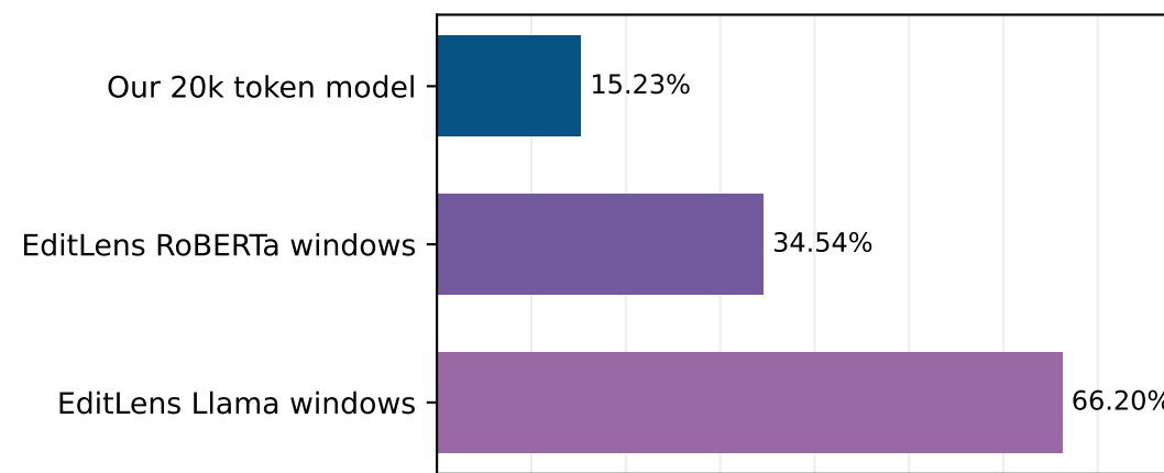
AITDNA mixed: human token FPR
