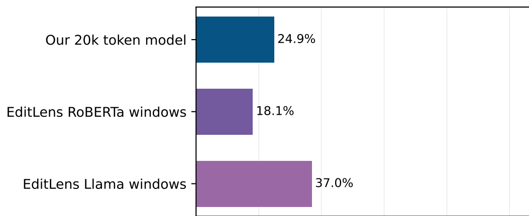
LLMTrace mixed: AI token recall
