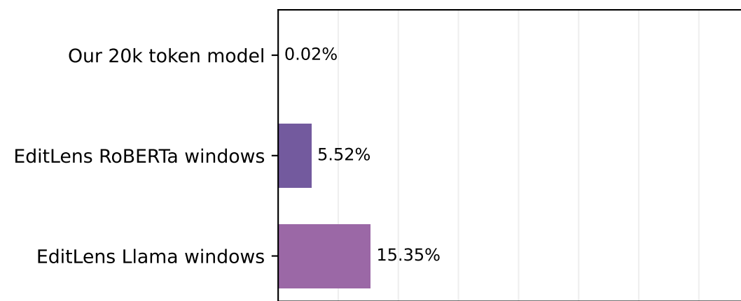
LLMTrace mixed: human token FPR
