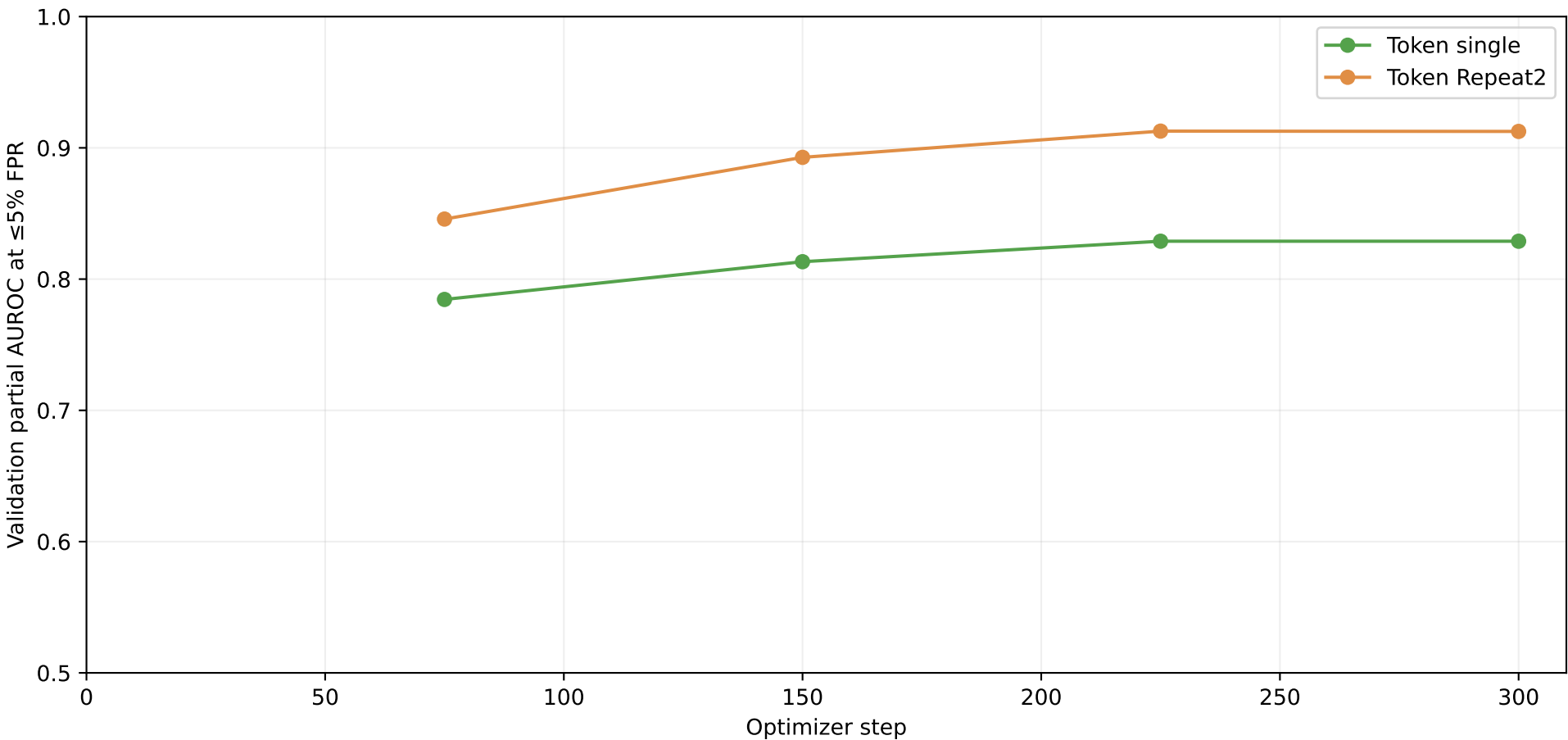
Token pilot learning curves
