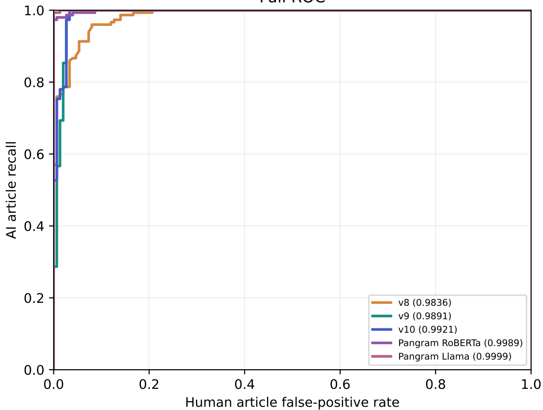
Full ROC
