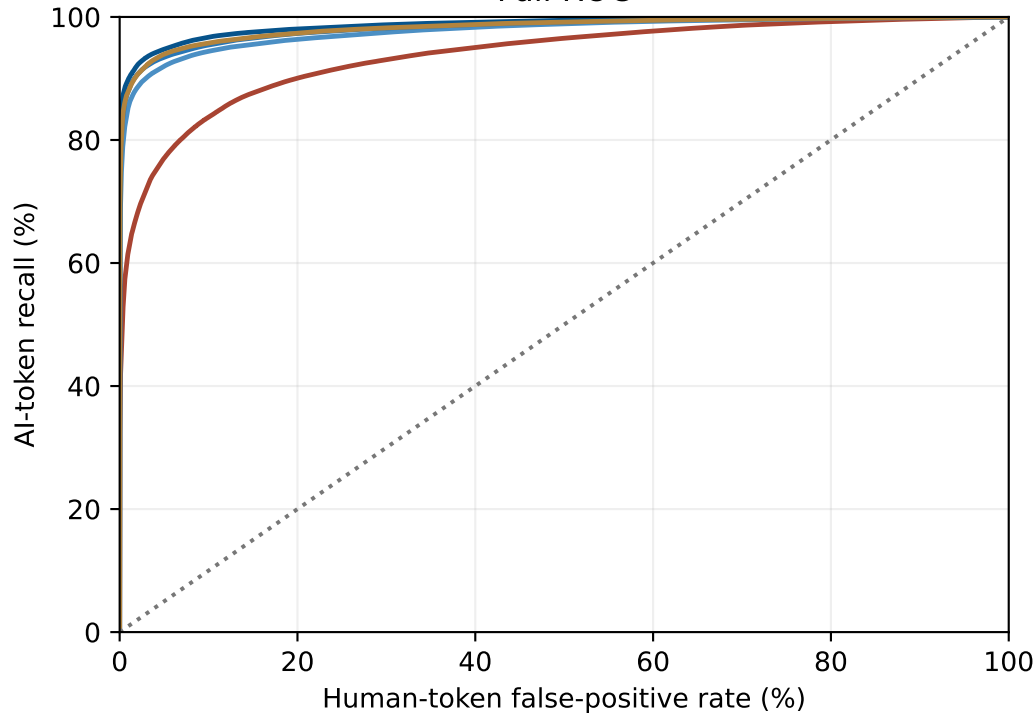
Full ROC
