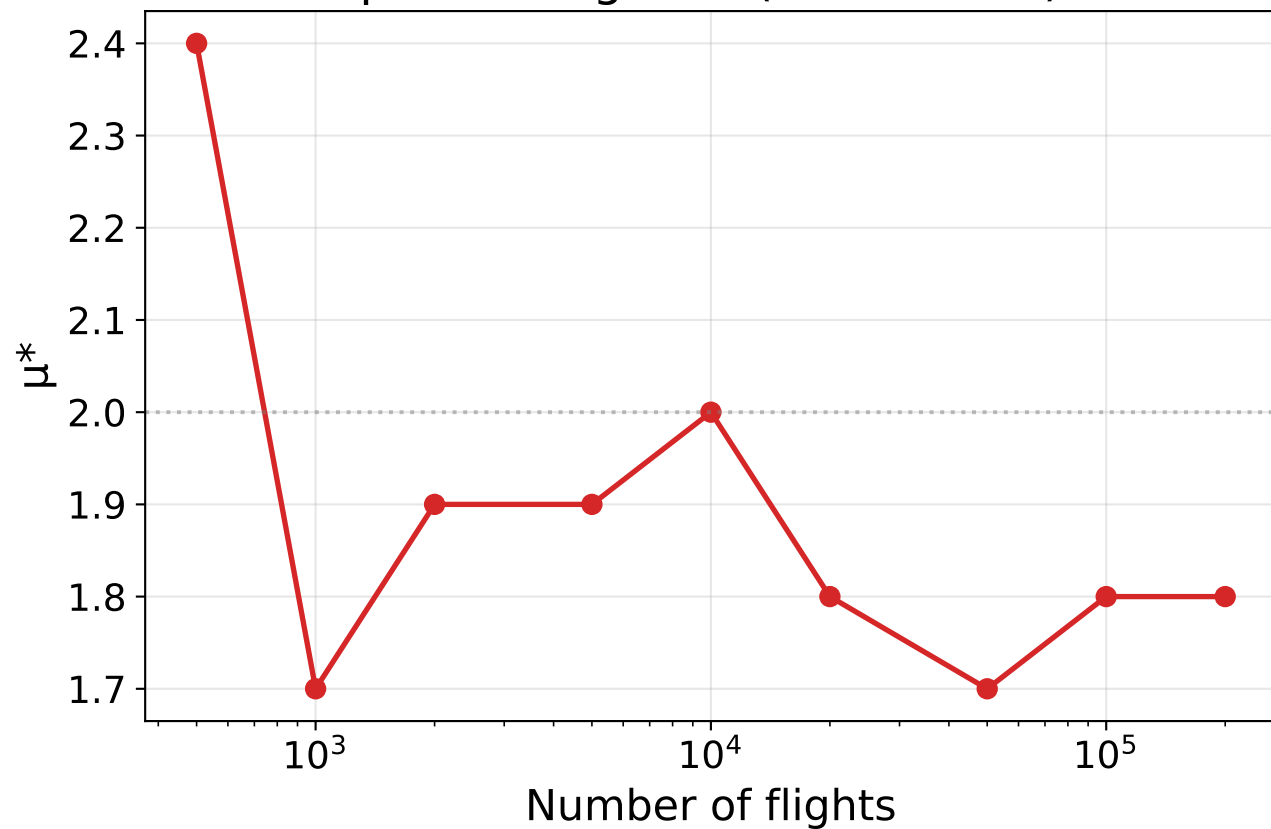
\mu^* convergence (destructive)
