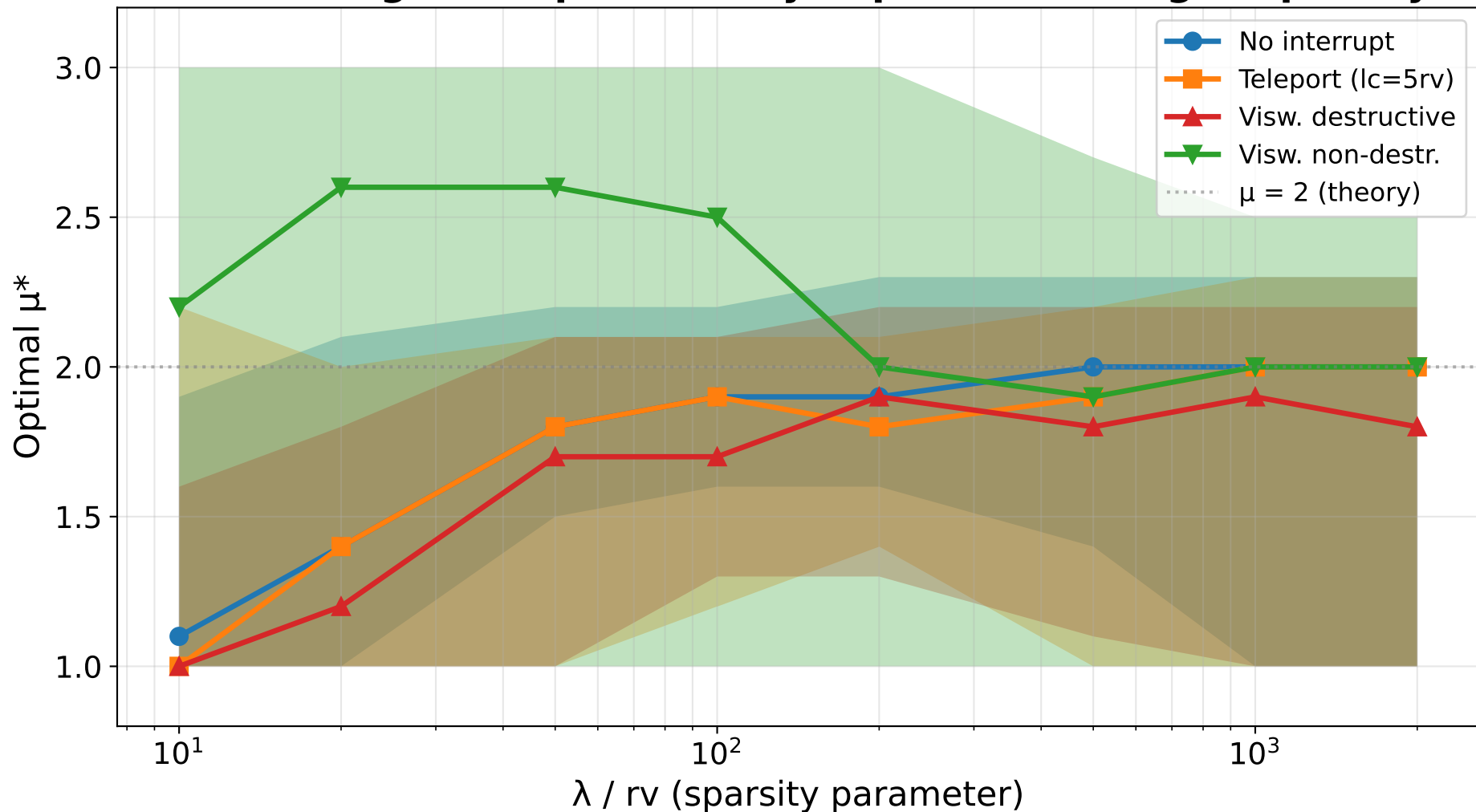
Phase Diagram: Optimal Lévy Exponent vs Target Sparsity
