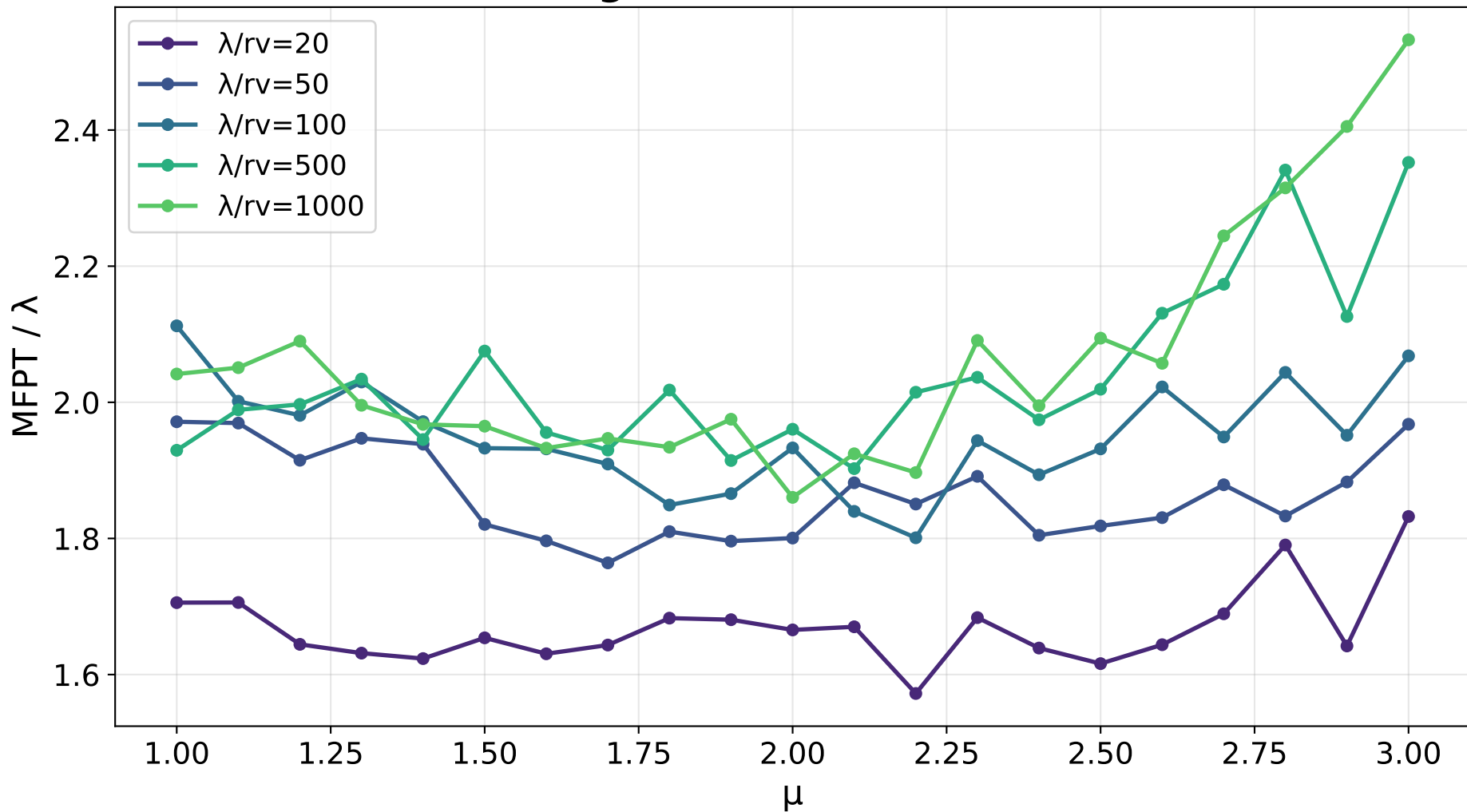
Mean First Passage Time (destructive Viswanathan)
