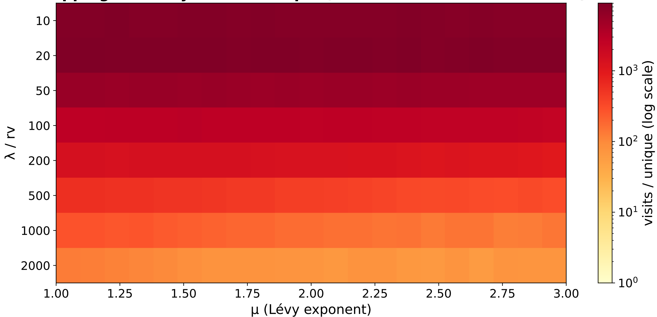
Trapping Intensity: visits / unique (Viswanathan non-destructive)
