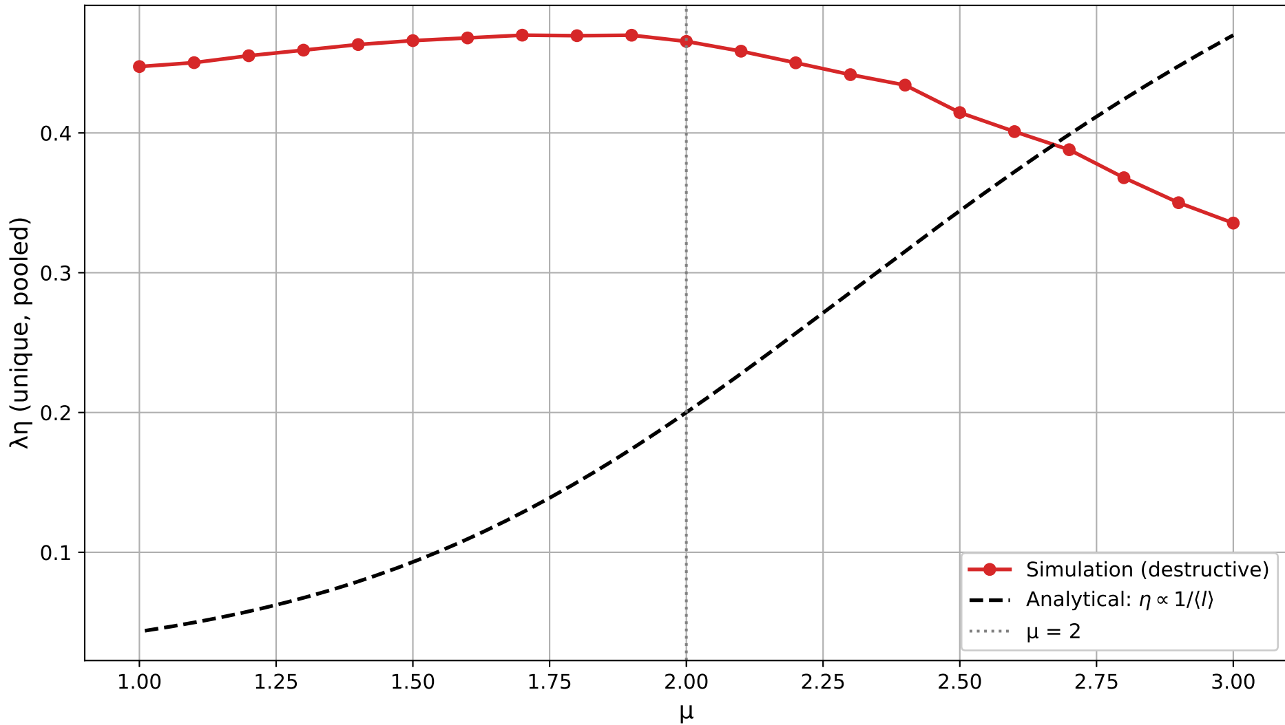
Comparison with Analytical Prediction ( \lambda/rv=100 )
