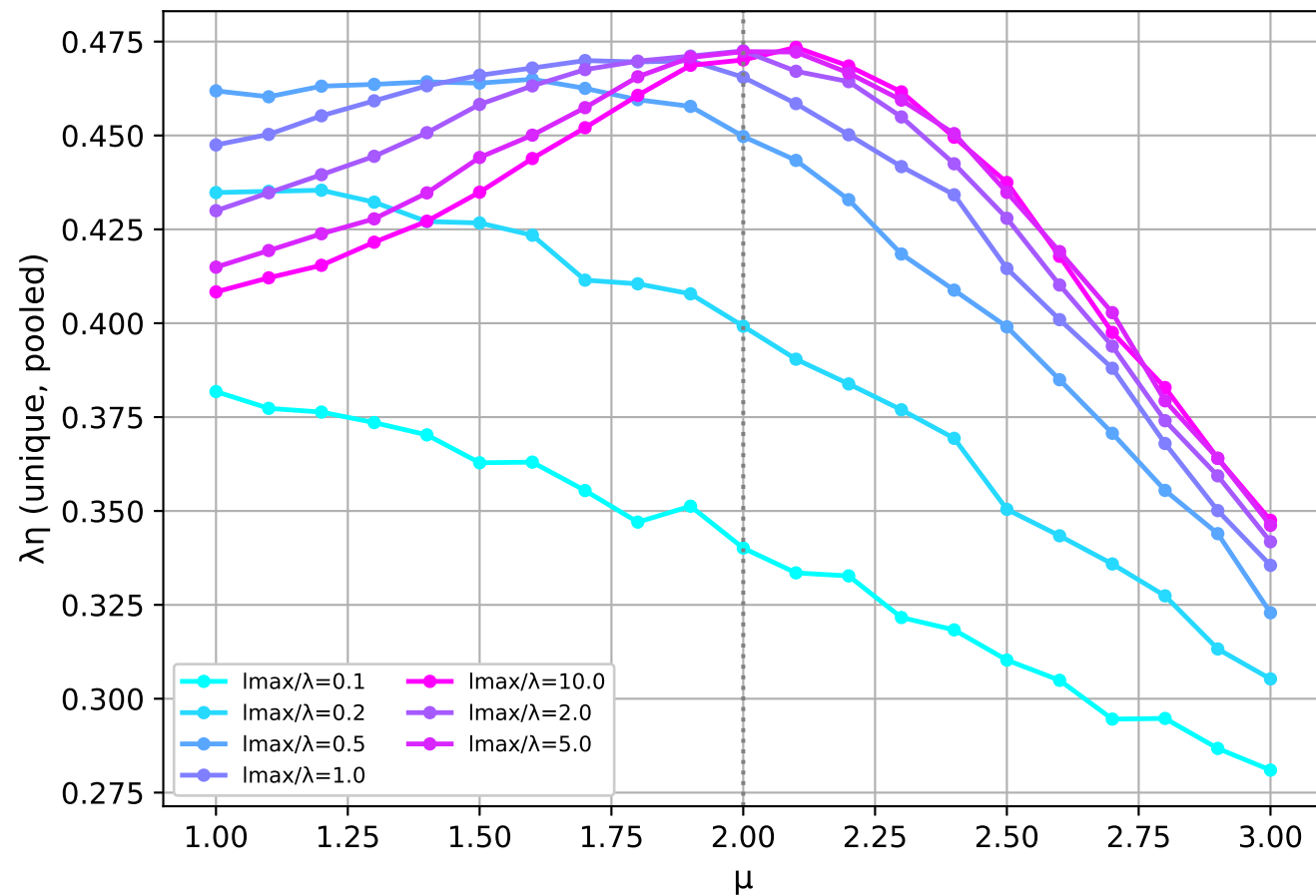
Effect of l_{\max} / \lambda
