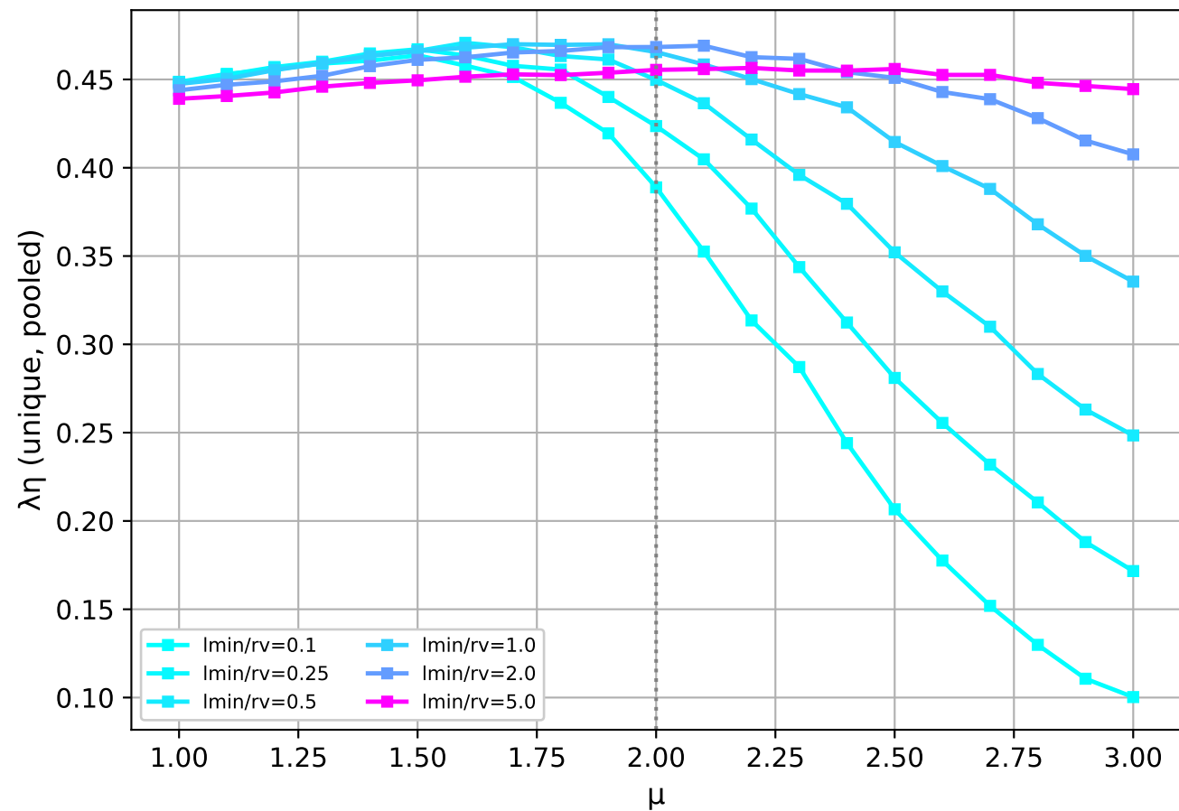
Effect of l_{\min} / rv
