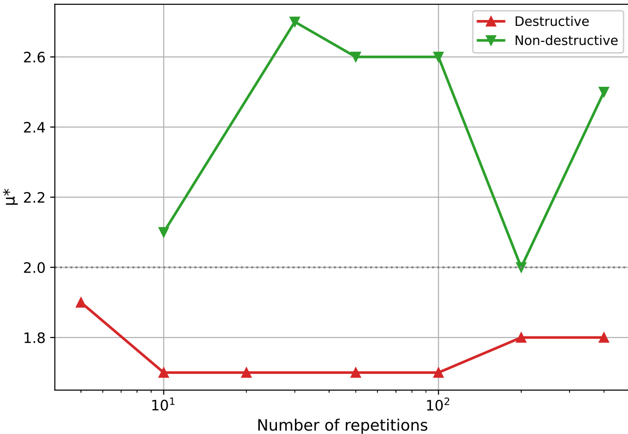
\mu^* convergence
