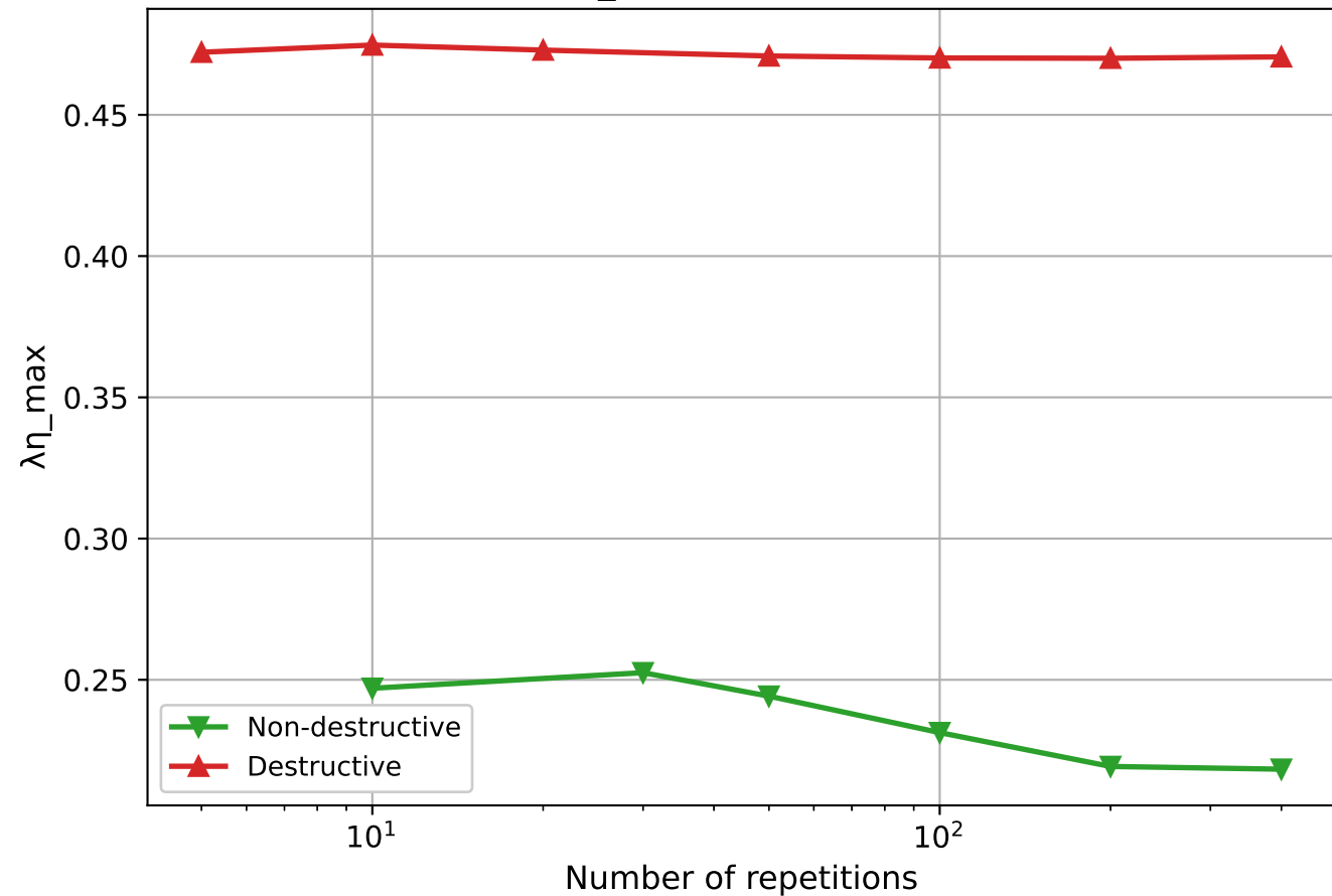
\lambda\eta_{\max} convergence
