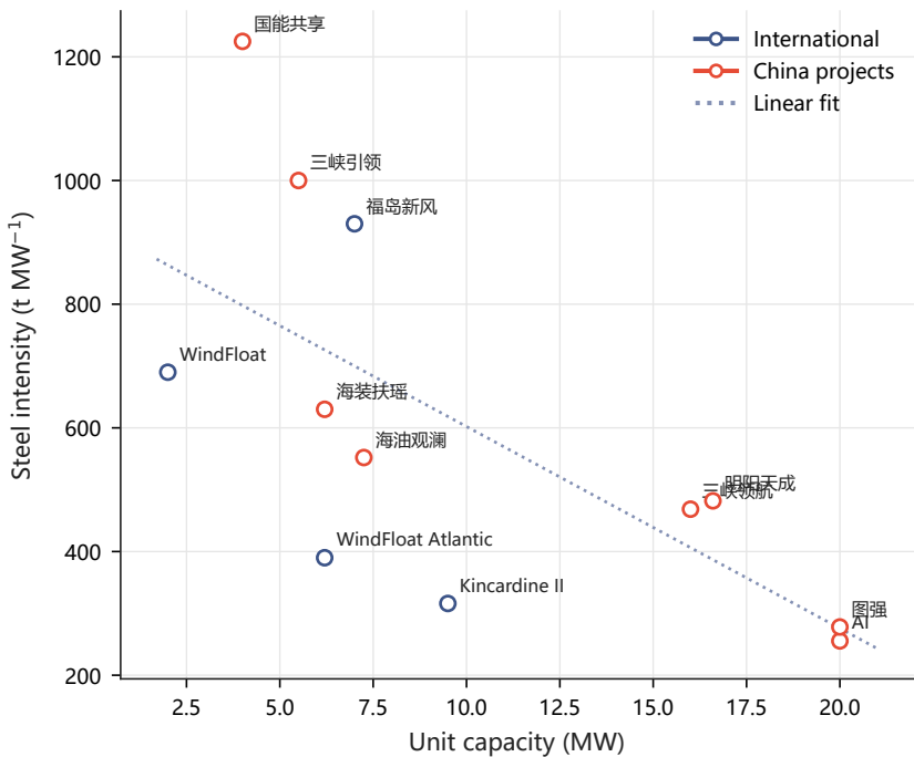
d Capacity vs. steel intensity
