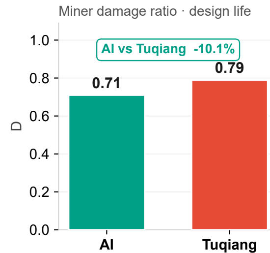
VII Component fatigue
