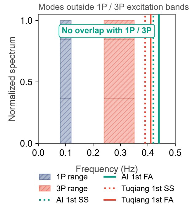
IV Structural frequency
