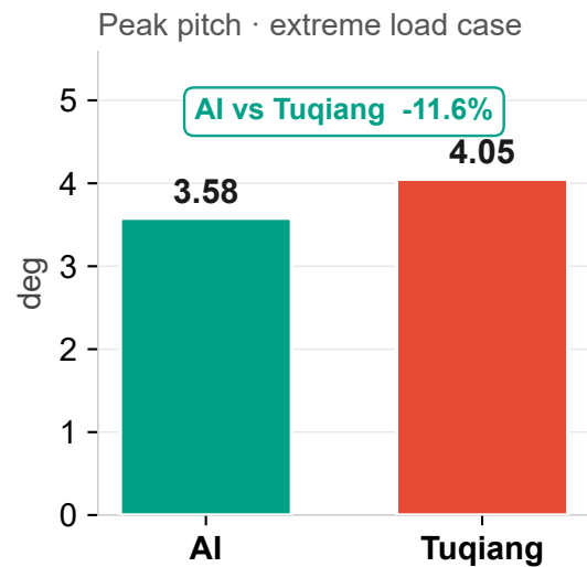
V Platform motion
