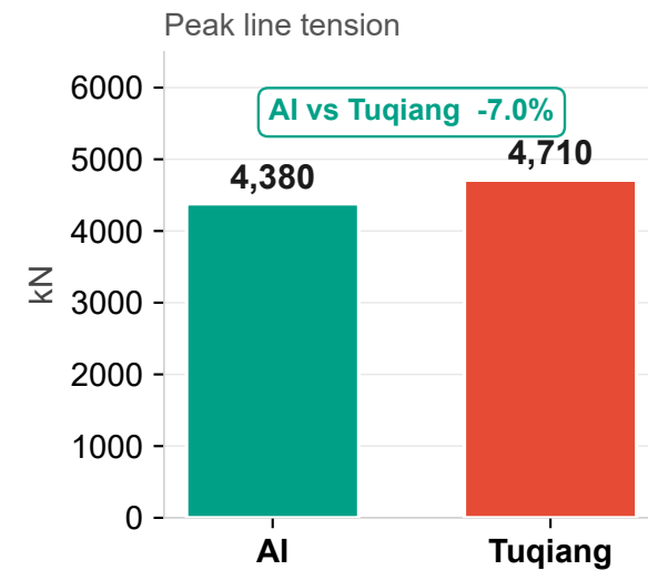
VIII Mooring tension
