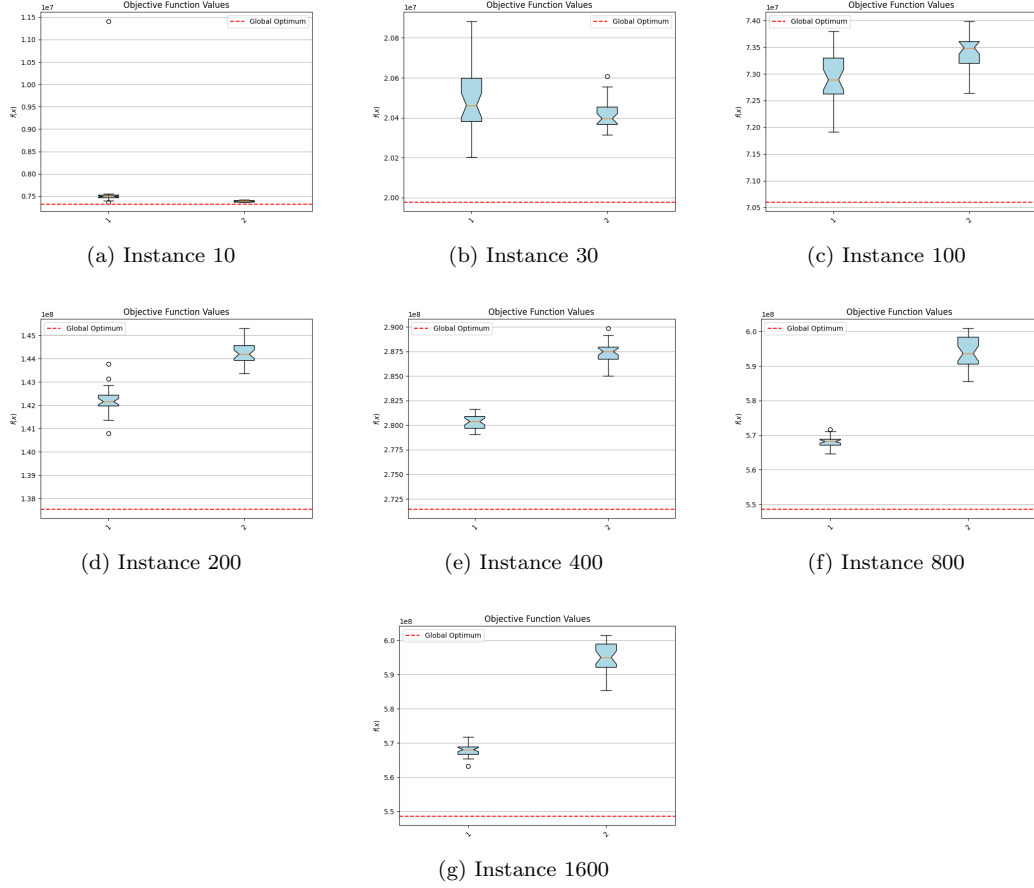
Figure 4: Distribution of objective function values for Proposed VNS (Novel) vs. Standard VNS (Basic) across all instance sizes. The novel approach demonstrates superior scalability.
