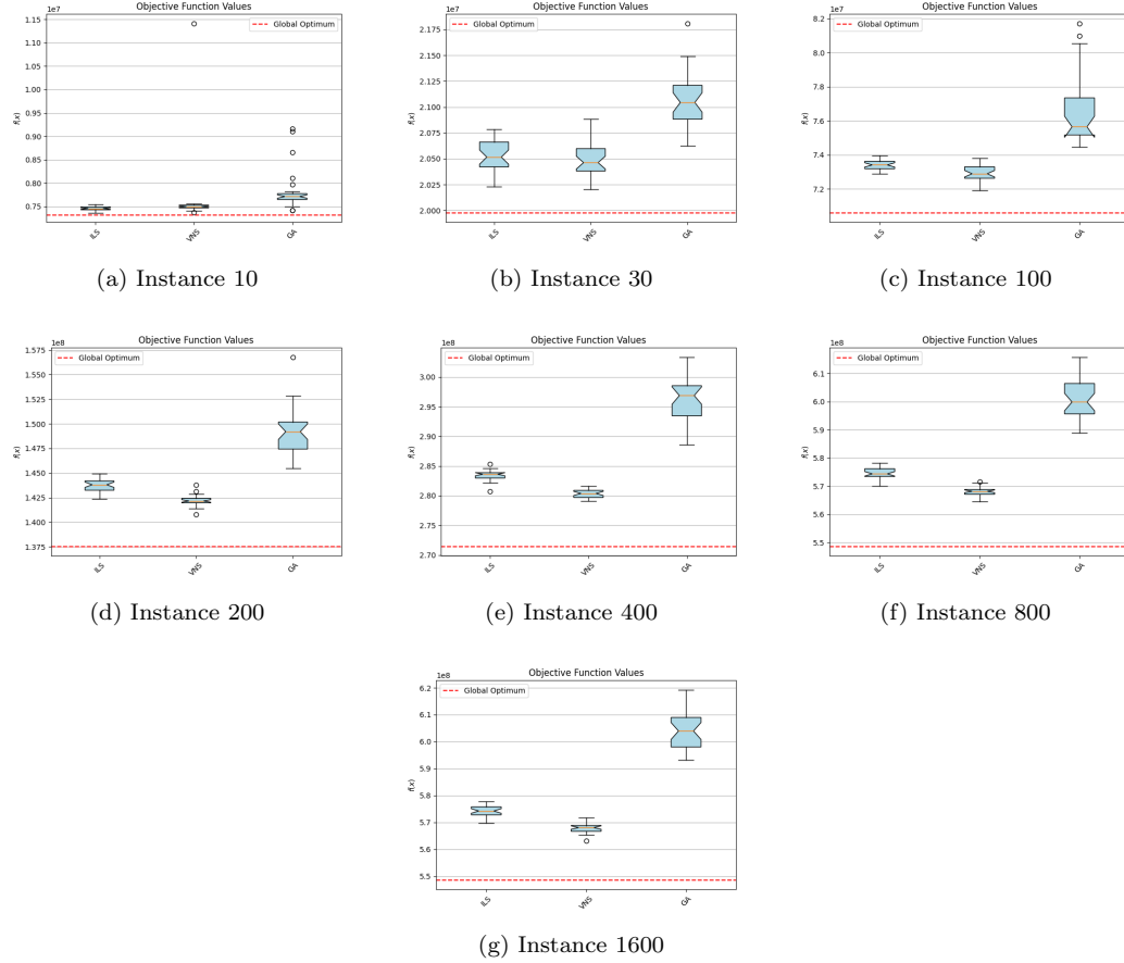
Figure 5: Comparison of VNS, ILS, and GA across all instance sizes. The red dashed line indicates the reference solution (Gurobi optimum or best incumbent).
