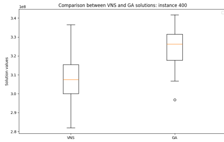
(c) I, J, K, E, S, Q, N1, N2, N3, M = 400
