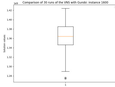
(e) I, J, K, E, S, Q, N1, N2, N3, M = 1600. The exact algorithm was not able to return a solution due to excessive resource demands.
