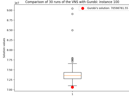
(a) I, J, K, E, S, Q, N1, N2, N3, M = 100
