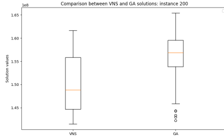
(b) I, J, K, E, S, Q, N1, N2, N3, M = 200
