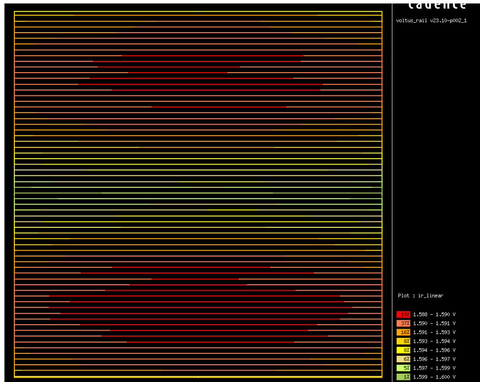
Figure 2. Commercial build: static IR map of VPWR (Voltus, vectorless): legend 1.588–1.600 V, worst drop 11 mV against an 80 mV budget.
