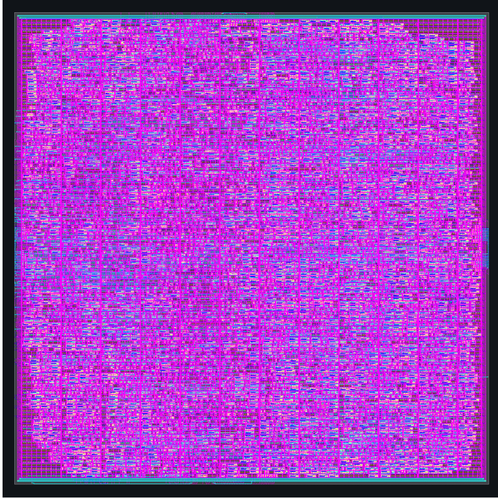
Figure 1. Commercial build: routed PicoRV32, 357.4 \times 355.6 \mu\text{m} , sky130A (KLayout render of the final GDS).
