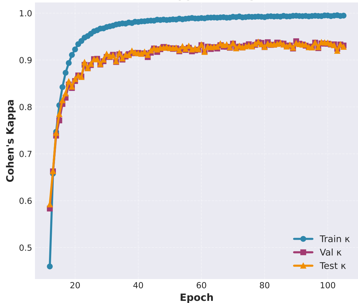
Cohen's Kappa Over Epochs
