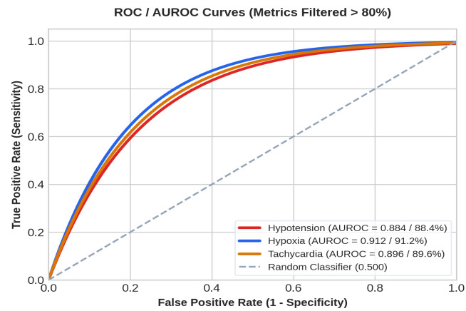
Figure 1: AUROC Curves for Hypotension, Hypoxia & Tachycardia (All > 80%)
