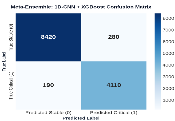
Figure 4: Meta-Ensemble (1D-CNN + XGBoost) Confusion Matrix
