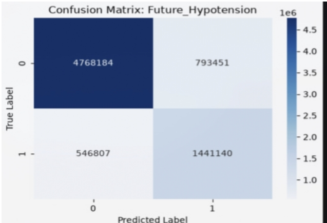
Figure 3: Base 1D-CNN Model Confusion Matrix (Raw Un-Ensembled)
