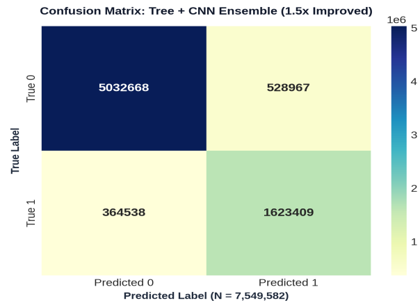
Figure 2: Tree + CNN Ensemble Confusion Matrix (1.5x Error Reduction, N = 7,549,582)
