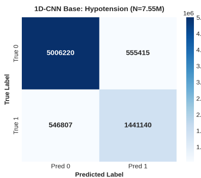
Figure 3: Base 1D-CNN Hypotension
