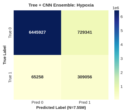
Figure 7: Tree+CNN Hypoxia (1.5x Improved)
