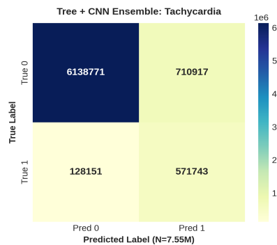
Figure 8: Tree+CNN Tachycardia (1.5x Improved)
