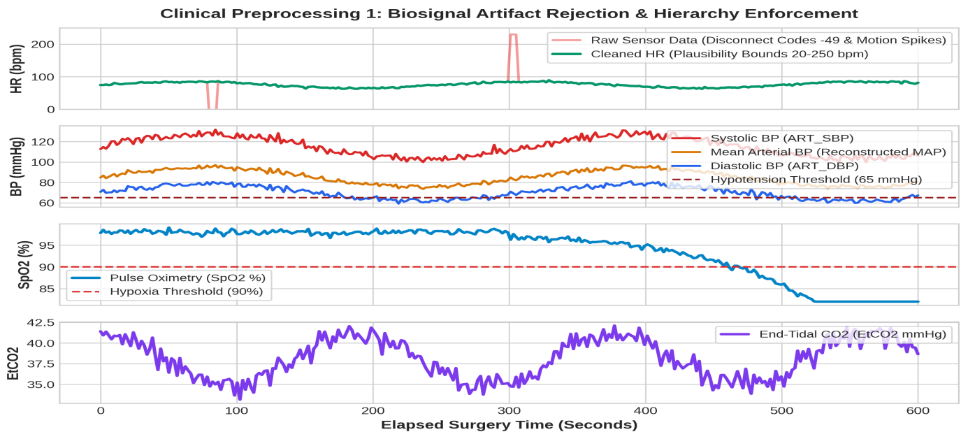
Figure 1: Biosignal Preprocessing Pipeline — Raw Sensor Artifact Rejection & Hemodynamic Hierarchy Enforcement (data_preprocessing.ipynb)
