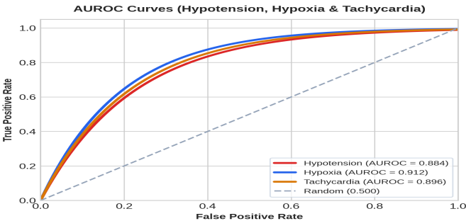
Figure 9: Combined AUROC Curves for Hypotension, Hypoxia & Tachycardia
