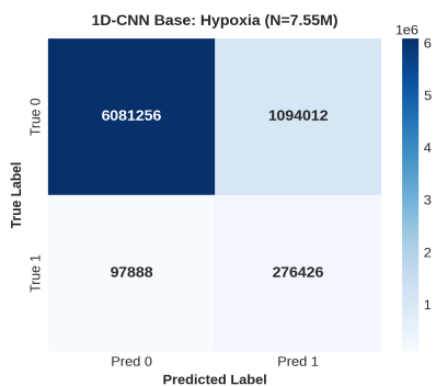
Figure 4: Base 1D-CNN Hypoxia
