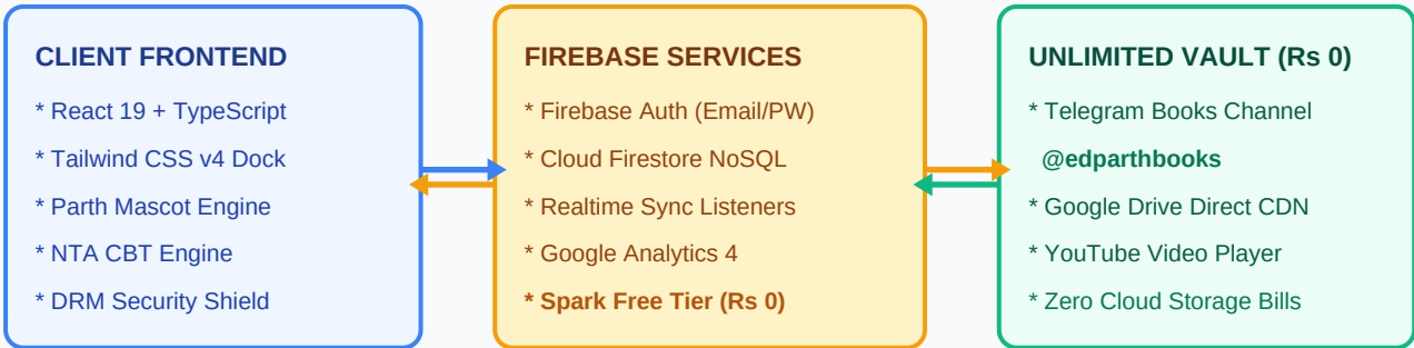
Figure 1: Full-Stack Cloud & Client Topology with Zero-Cost Storage Architecture
