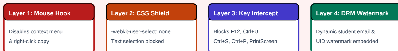
Figure 6: 4-Layer Enterprise DRM & Anti-Piracy Guard Protecting Platform Content
