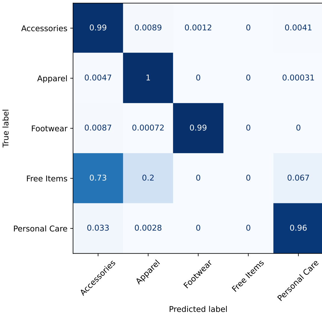
MobileNetV2 - Normalised Confusion Matrix
