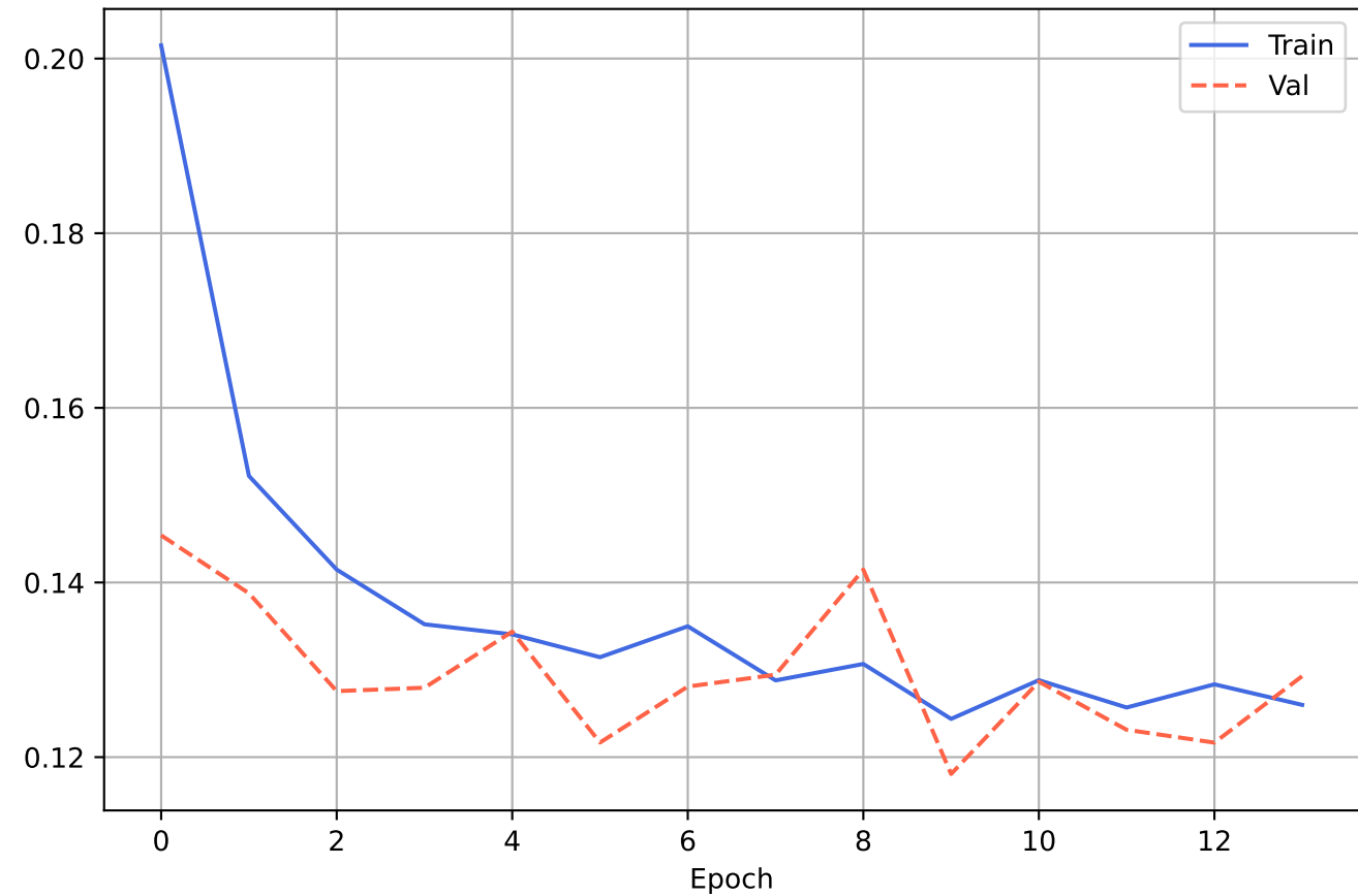
MobileNetV2 - Loss
