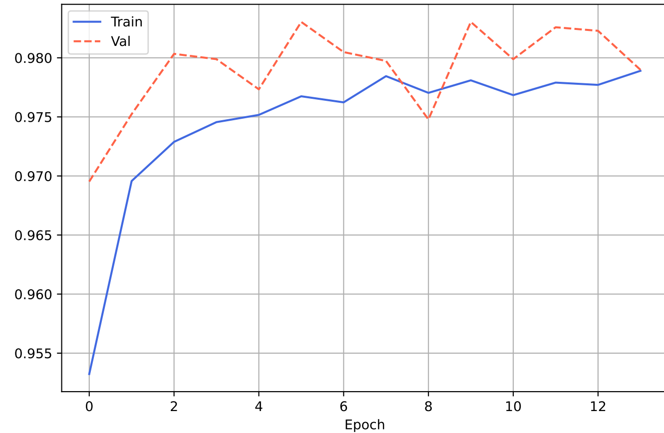
MobileNetV2 - Accuracy
