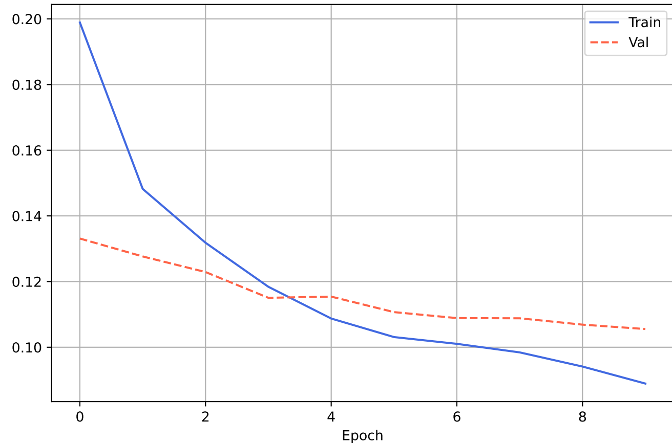
MobileNetV2 Fine-Tuned - Loss
