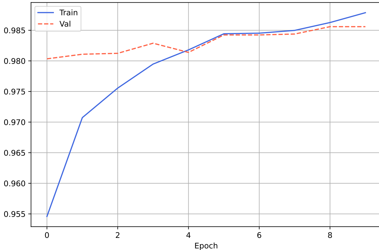
MobileNetV2 Fine-Tuned - Accuracy
