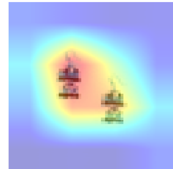
Pred: Accessories
