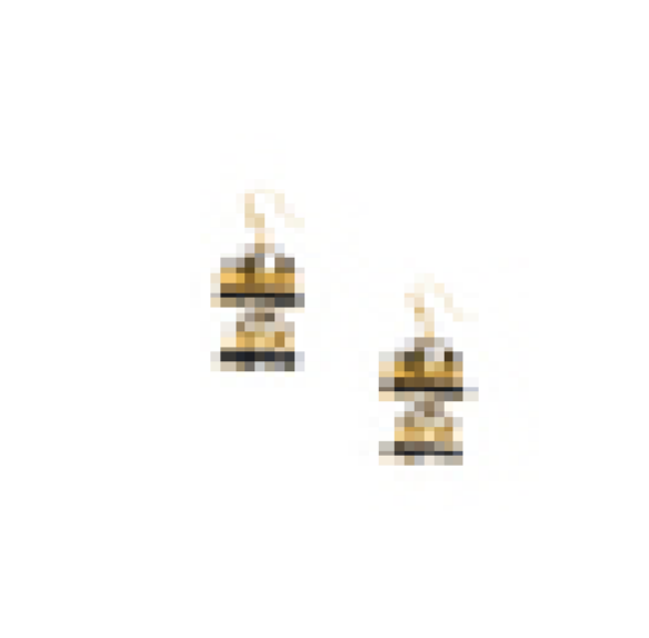
Pred: Accessories
