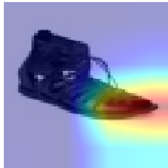
Pred: Footwear
