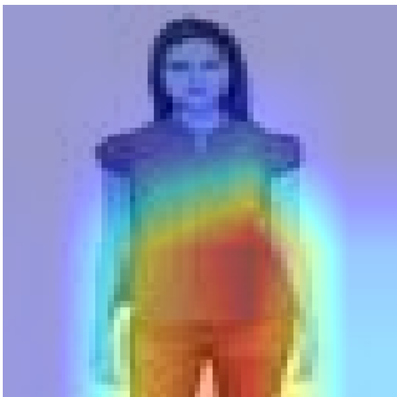
Pred: Apparel
