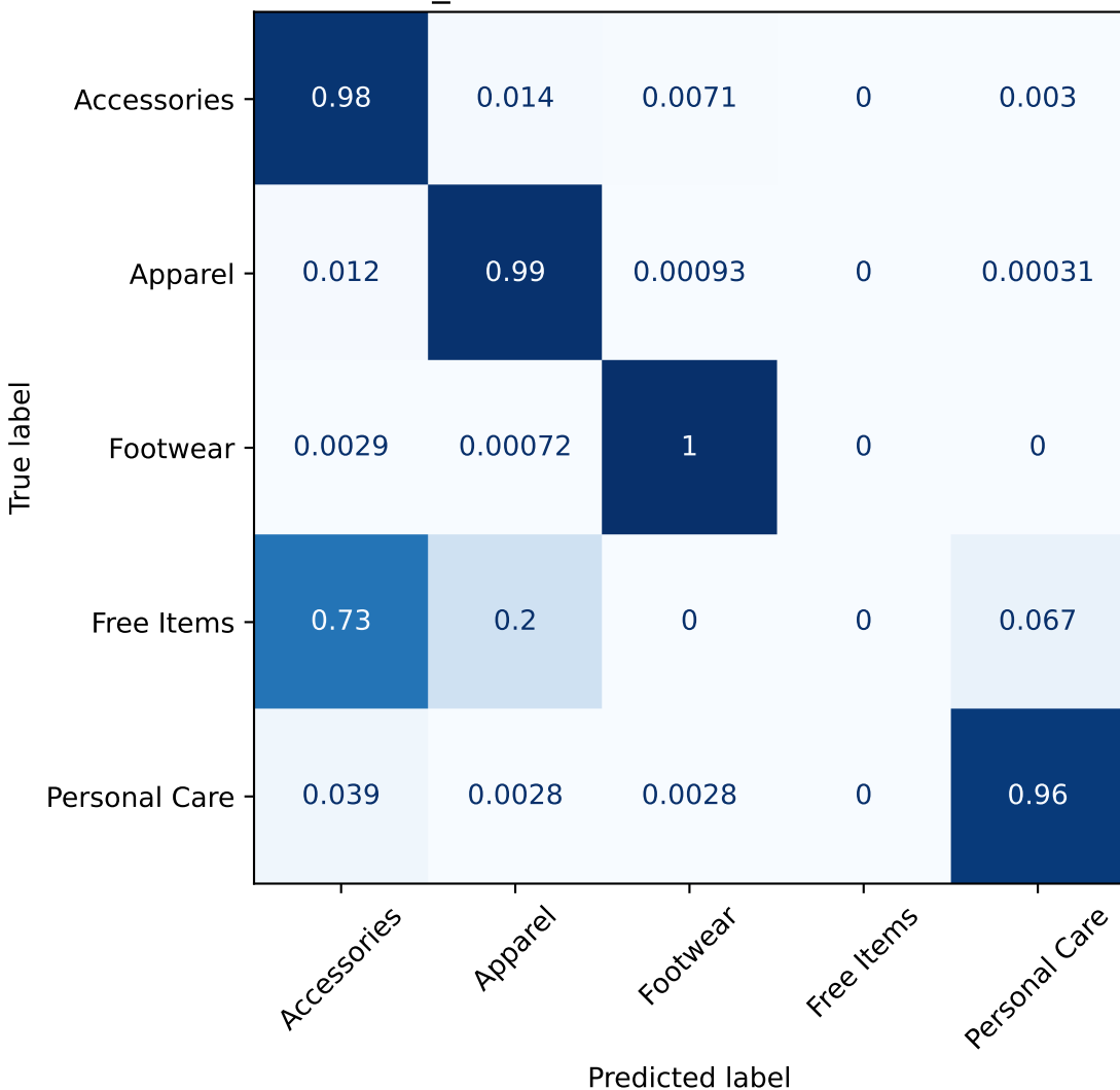
Custom_CNN - Normalised Confusion Matrix
