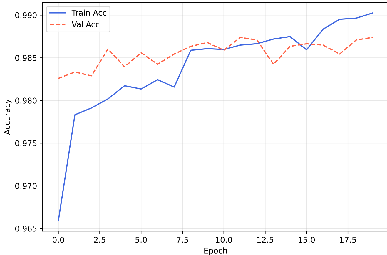
EfficientNetB0 - Accuracy
