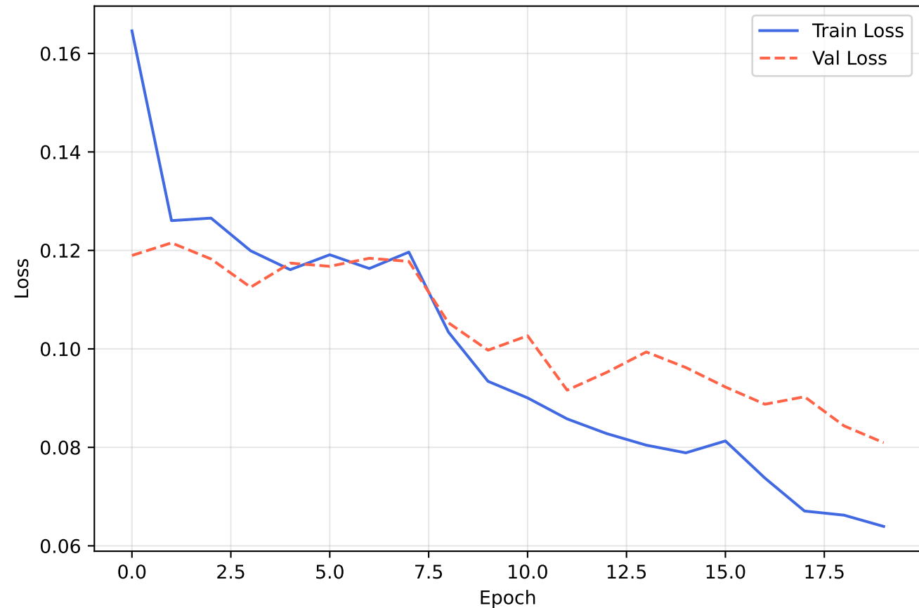
EfficientNetB0 - Loss
