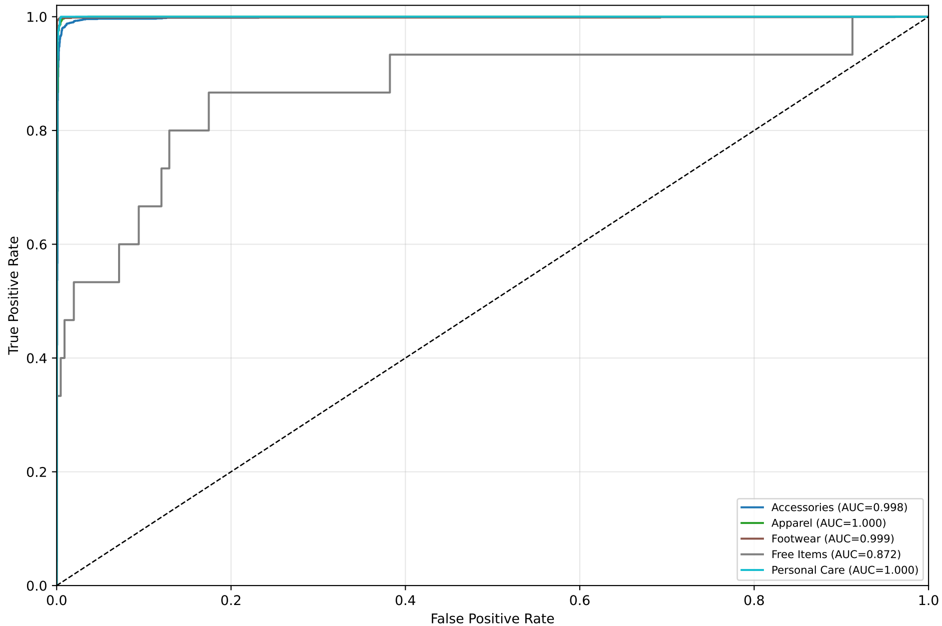
MobileNetV2 - ROC Curves (One-vs-Rest)
