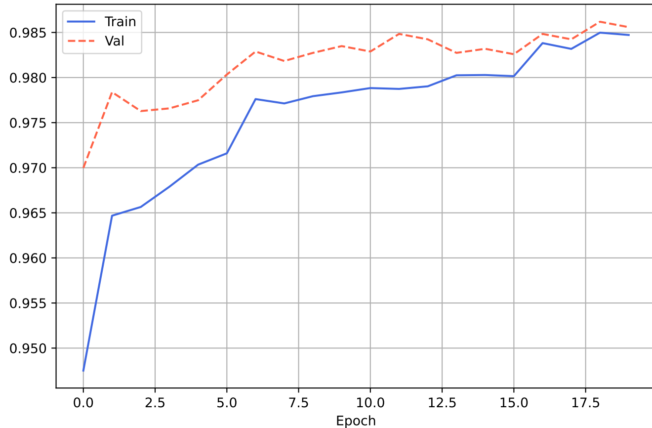
ResNet50 - Accuracy
