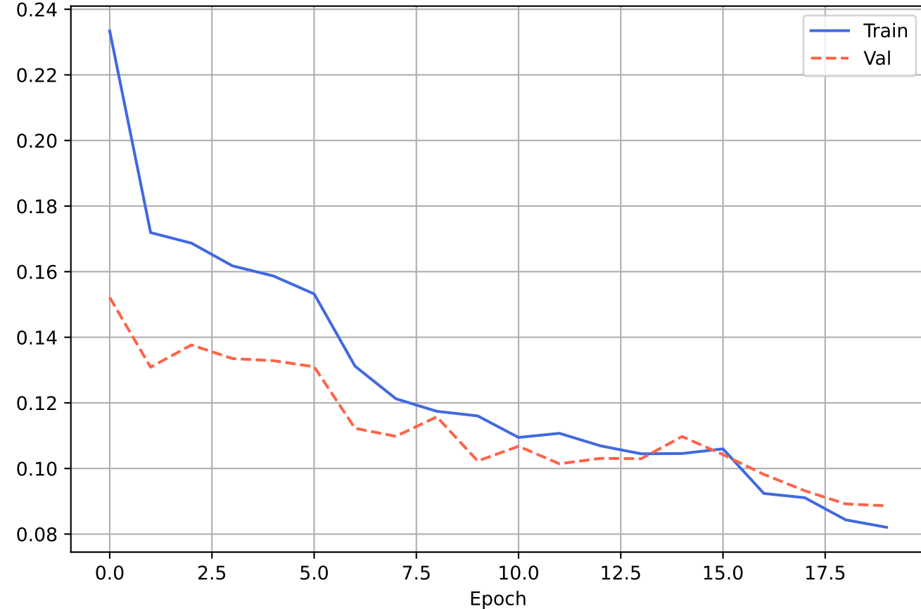
ResNet50 - Loss
