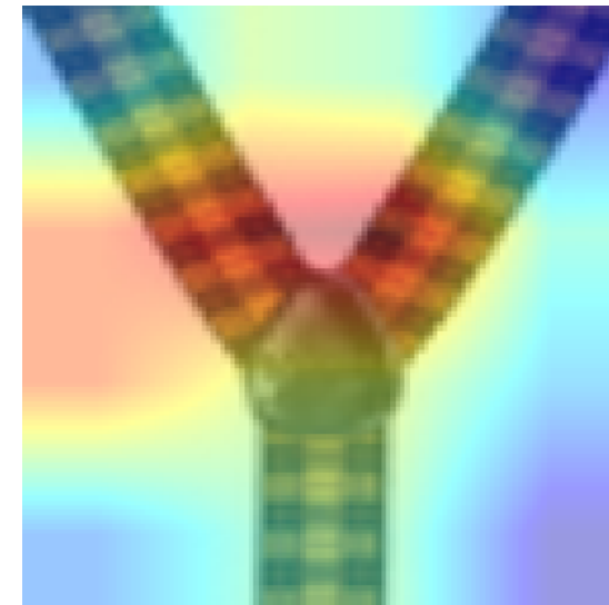
Pred: Accessories
