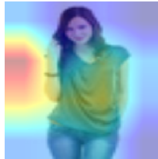
Pred: Accessories
