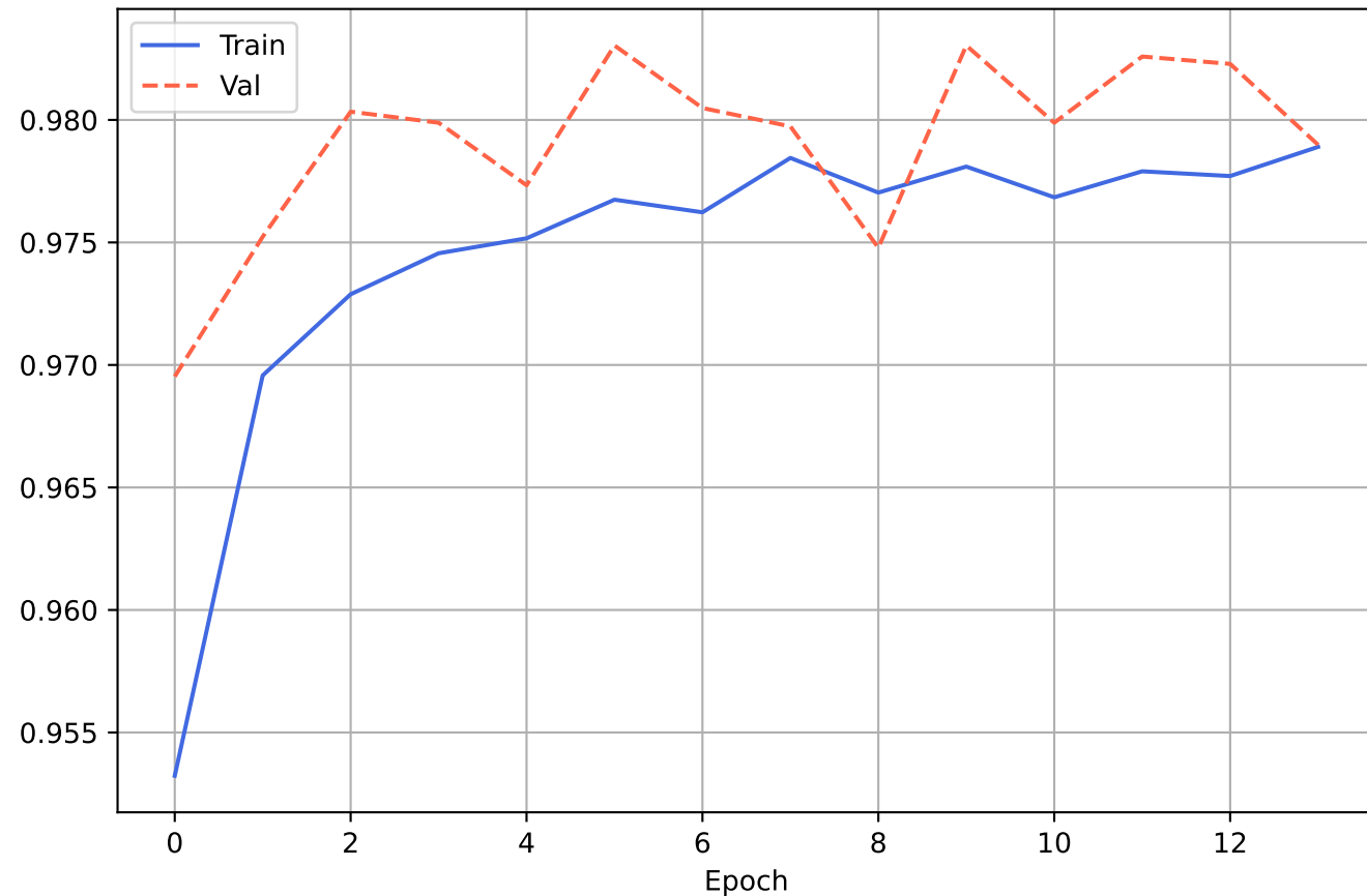
MobileNetV2 - Accuracy
