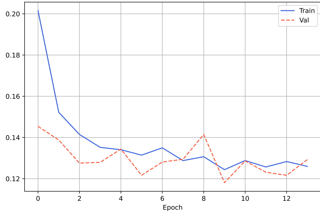
MobileNetV2 - Loss
