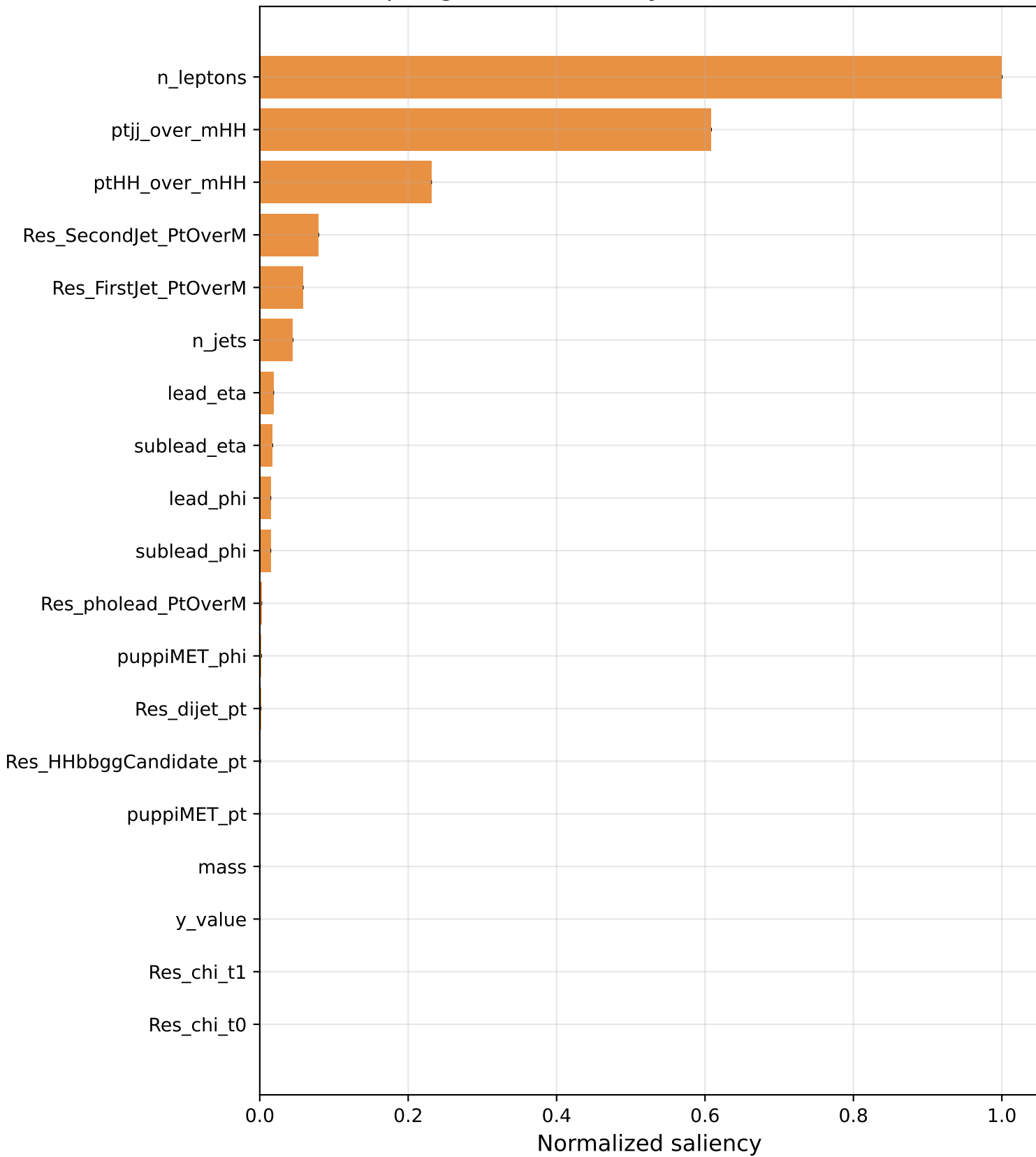
Input-gradient saliency (normalized) -- TEST
